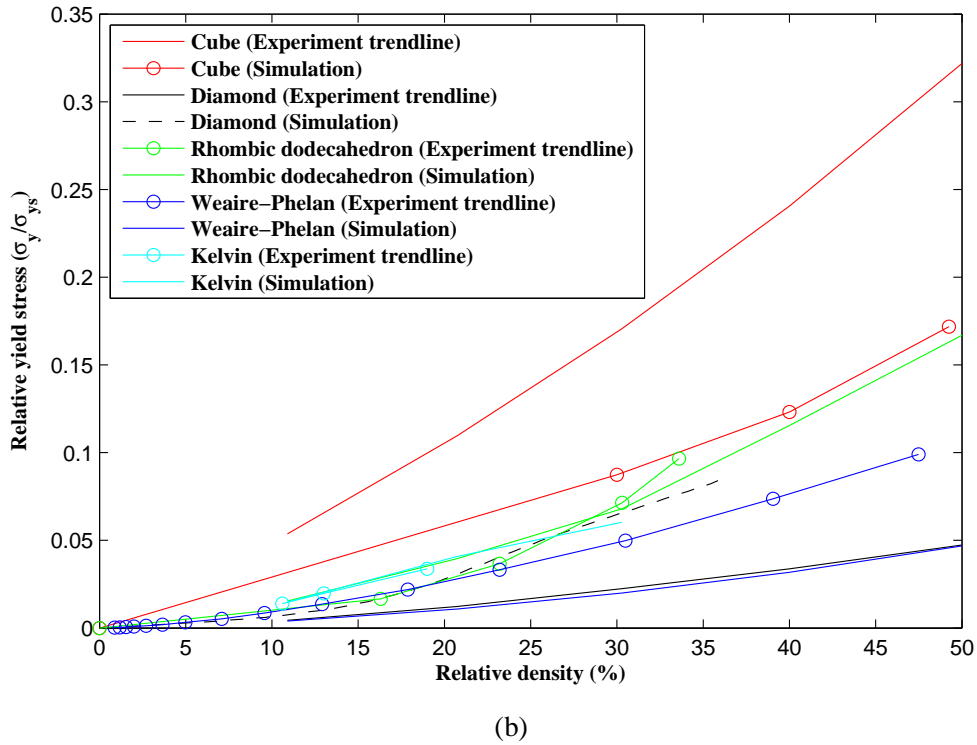
Figure 4- Comparison of numerical and experimental (a) elastic modulus and (b) yield stress for the unit cell types considered in this study
