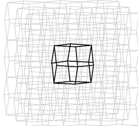
Rhombic dodecahedron
