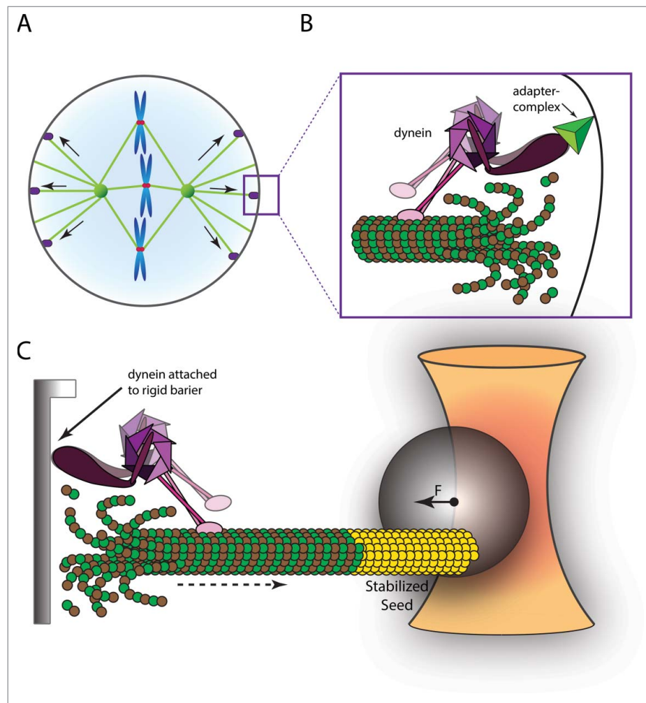
Figure 3. Pulling forces generated by depolymerising microtubules drive spindle positioning. (A) Mitotic spindle positioning is accomplished by linking depolymerizing microtubules to the cell cortex. (B) Dynein (purple) is anchored to the cell cortex by means of the NuMa/LGN/G \alpha i trinary adapter complex (green) and interacts with shrinking microtubules. (C) Single molecule approach to study dynein-mediated pulling forces using an optical trap setup. Barrier (gray) attached dynein is bound to a depolymerizing microtubule that has grown from a stabilised seed (yellow) that has been linked to a magnetic bead (gray sphere). The formation of load-bearing attachments results in a pulling force (F) that displaces the bead from the optical trap (yellow).
