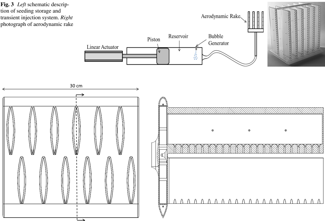
Fig. 4 Scale drawing of aerodynamic rake with 12 bi-convex airfoils staggered in two rows and with 264 orifices. Left top view; right section view
