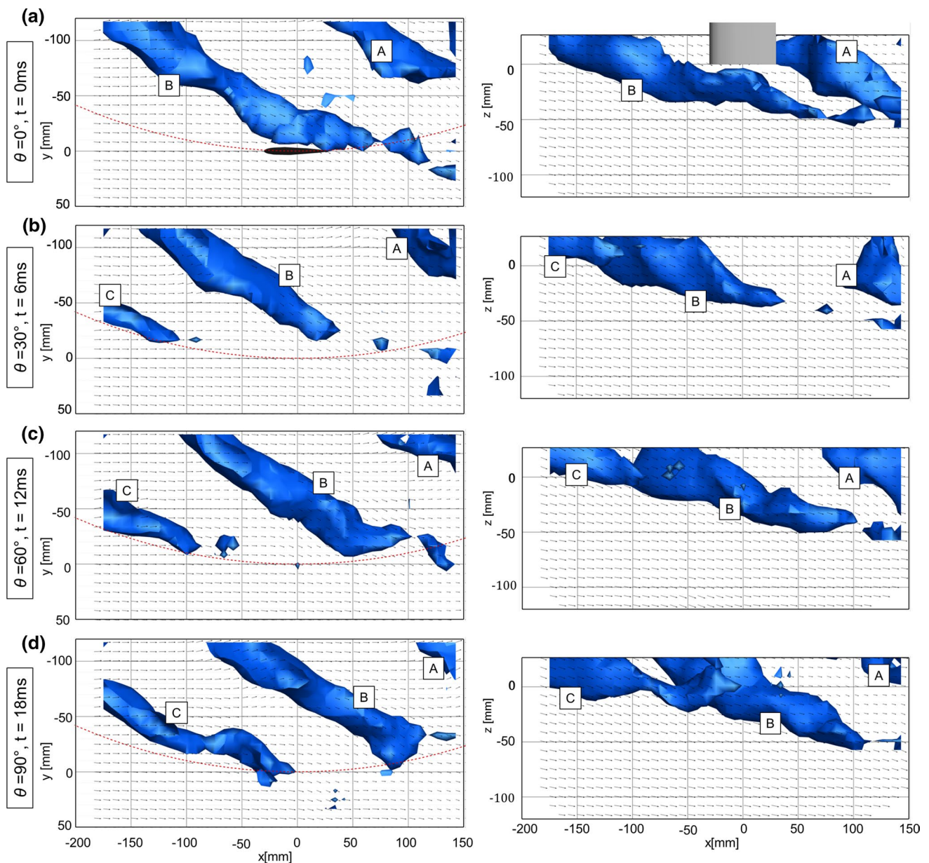
Fig. 9 Instantaneous velocity vector field (from cross-correlation) and vorticity magnitude iso-surface ( |\omega| = 170/\text{s} ) for tip vortices generated by the retrograding blade in a VAWT. One plane of velocity
