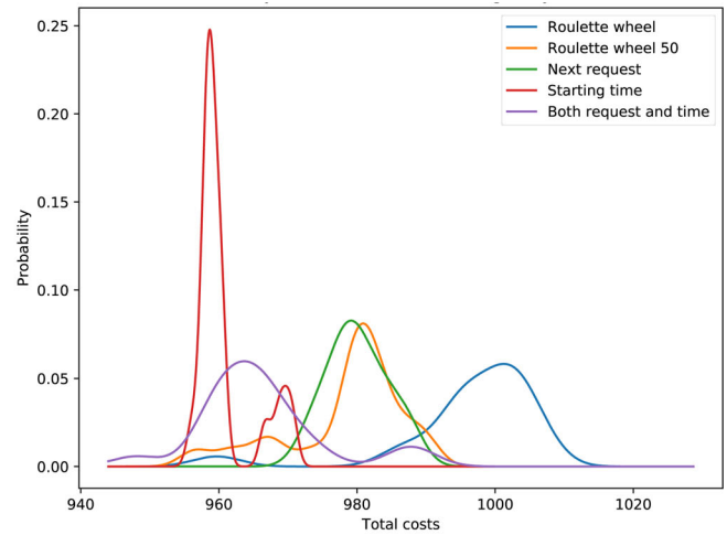
(b) Kernel density estimation, costs only
