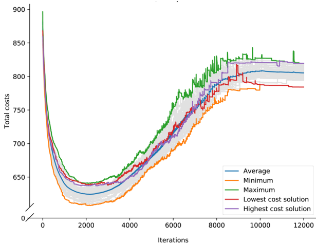
FIGURE 4 ES robustness analysis, Year X data
