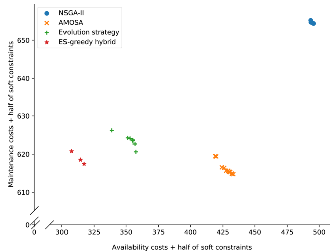
(b) Pareto frontier between cost types: ES, hybrid, and two multi-objective GAs. Year X data.
