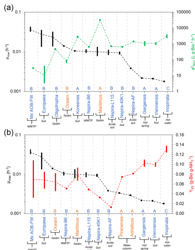
FIGURE 1 Maximum specific growth rate ( \mu_{max} ) with (a) specific affinity for ammonia ( a^0_{NH_3} ) and (b) growth yield ( Y_{XS} ) of ammonia-oxidizing microorganisms (AOB, AOA, and CMX). The black bars show the range of \mu_{max} values; green bars represent the range of a^0_{NH_3} value for ammonia (a); and red bars represent the range of Y_{XS} values (b). Blue: non-marine nitrifiers; orange: marine nitrifiers. Legend bottom of figures: B – Bacteria; A – Archaea; C – Complete ammonia oxidizer. Dashed lines cross the calculated average value for each parameter function of the range of values reported
