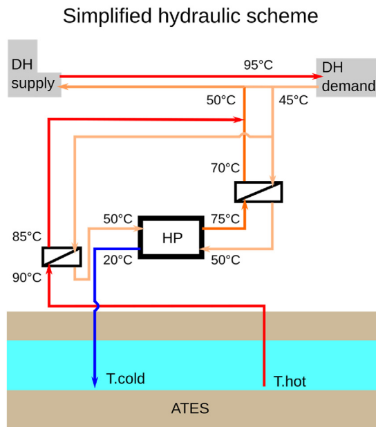
Fig. 3. HT-ATES and HP integration schematic representation integration for the case of 20 °C re-injection temperature and the respective energy conversions related to the HP. Notice that to enhance the system efficiency, the HT-ATES and the HP production are injected in the DHN return branches.
