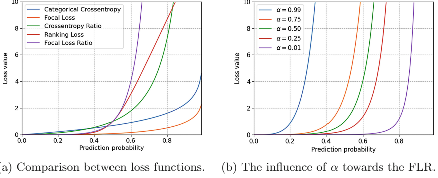
Fig. 1. Demonstration of different loss functions.
