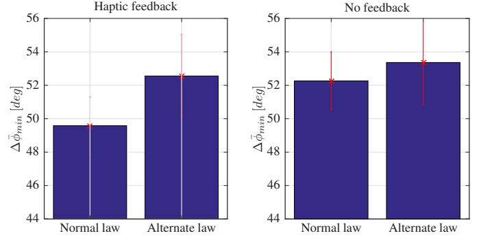
Fig. 10. Bank margin in the icing scenario.
