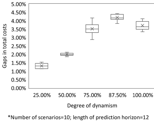
Fig. 5 Impact of the degree of dynamism
