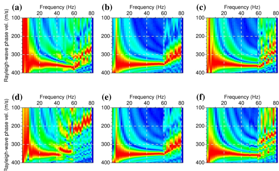
Figure 16: Comparison of Rayleigh-wave dispersion images for preprocessed field data, computed data from the initial model, and computed data from the inverted model. (a) Dispersion image calculated from the preprocessed common-source gather shown in Figure 14a, the source is located at x = 14.5 m; (b) dispersion image from the computed data using the initial model shown in Figure 12a; (c) dispersion image from the computed data using the inverted model shown in Figure 12b. (d), (e), (f) are same as (a), (b), (c) but for a common-source gather with the source located at x = 29.5 m.
