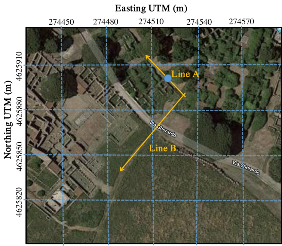
Figure 07: Photo of an unexcavated area in the ancient Ostia (from Google map). The two seismic lines A and B are indicated by yellow lines, where the arrows point in the direction of increasing coordinates (directions in which the source was moved) along the x-axes \cite[]{}{Ghose_2020}. The blue dot marks the approximate location of a tumulus identified earlier. Note that there are ancient walls present not too far away from the seismic lines.
