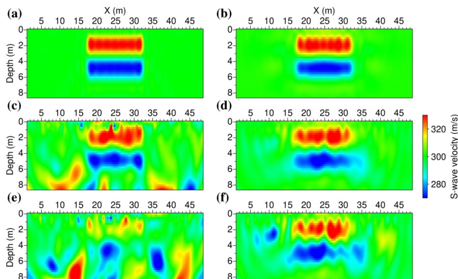
Figure 06: Test of inversion robustness to random noise present in the data. To maintain consistency with the checkerboard tests illustrated in Figure 3, the same bandpass filter (10 to 60~Hz) is applied to the data in Figure 5. (a) Inverted V_S model by least-squares FWI using noise-free synthetic data; (c) the same as (a) but for data contaminated by random noise with S/N = 20; (e) the same as (a) but for data contaminated by random noise with S/N = 10. (b), (d), (f) are the same as (a), (c), (e), respectively, but using instantaneous-phase coherency FWI.
