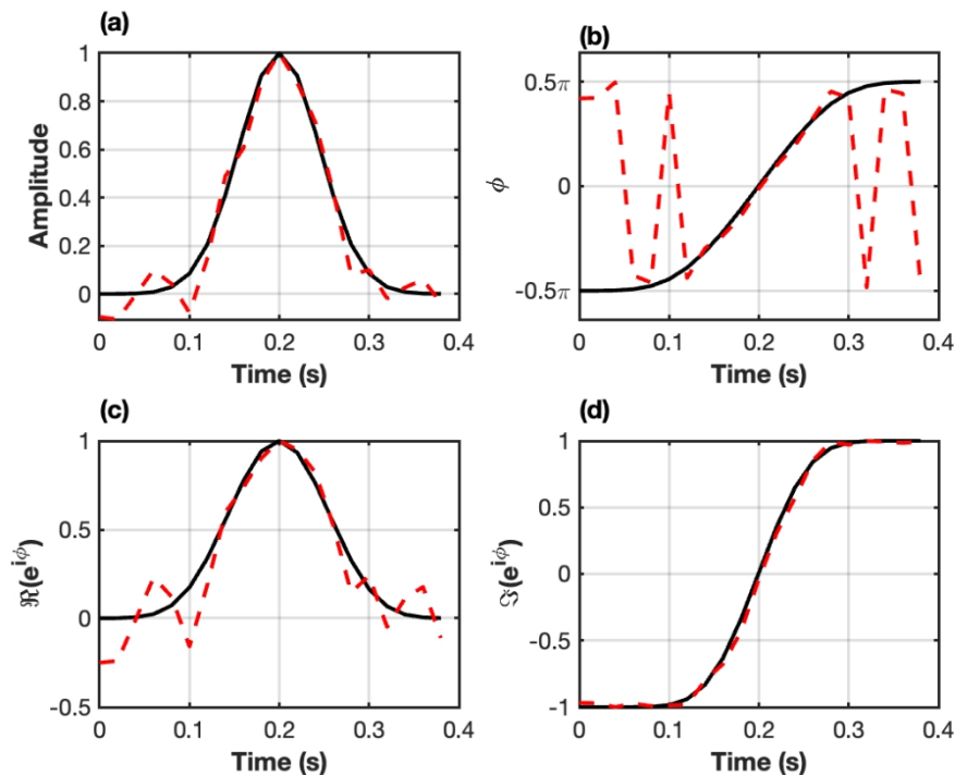
Figure 02: A simple synthetic example to demonstrate the robustness to noise of instantaneous phase ( \phi(t) ) and exponentiated phase ( e^{i\phi(t)} ). (a) A Gaussian signal with a peak frequency of 5 Hz (black line) and the same Gaussian signal with random noise and S/N = 10 (red-dashed line). In (b), (c), (d), we use black and red-dashed lines to represent respectively the instantaneous phase and exponentiated phase of the two signals presented in (a). (b) The instantaneous phase of the two signals as presented in (a). Note that for the signal with random noise, there are marked phase jumps. (c) The real part of the exponentiated phase of the two signals presented in (a). (d) The imaginary part of the exponentiated phase of the two signals presented in (a). Comparing (c), (d) with (b), it is clear that the exponentiated phase is more robust to noise.
