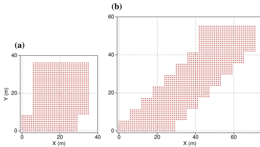
Figure 08: Layout of the receiver arrays used to acquire 2D seismic data along (a) seismic line A and (b) seismic line B, marked in Figure 7. For seismic lines A and B, the receiver interval is 0.25 m, while the source interval is 1 m. The number of common-source gathers acquired along seismic lines A and B are 37 and 57, respectively. The x-axis denotes the lateral positions of receivers, the y-axis represents the corresponding source positions for each receiver. The small, red triangles represent vertical, single-component geophones. Every fourth receiver position is displayed here.
