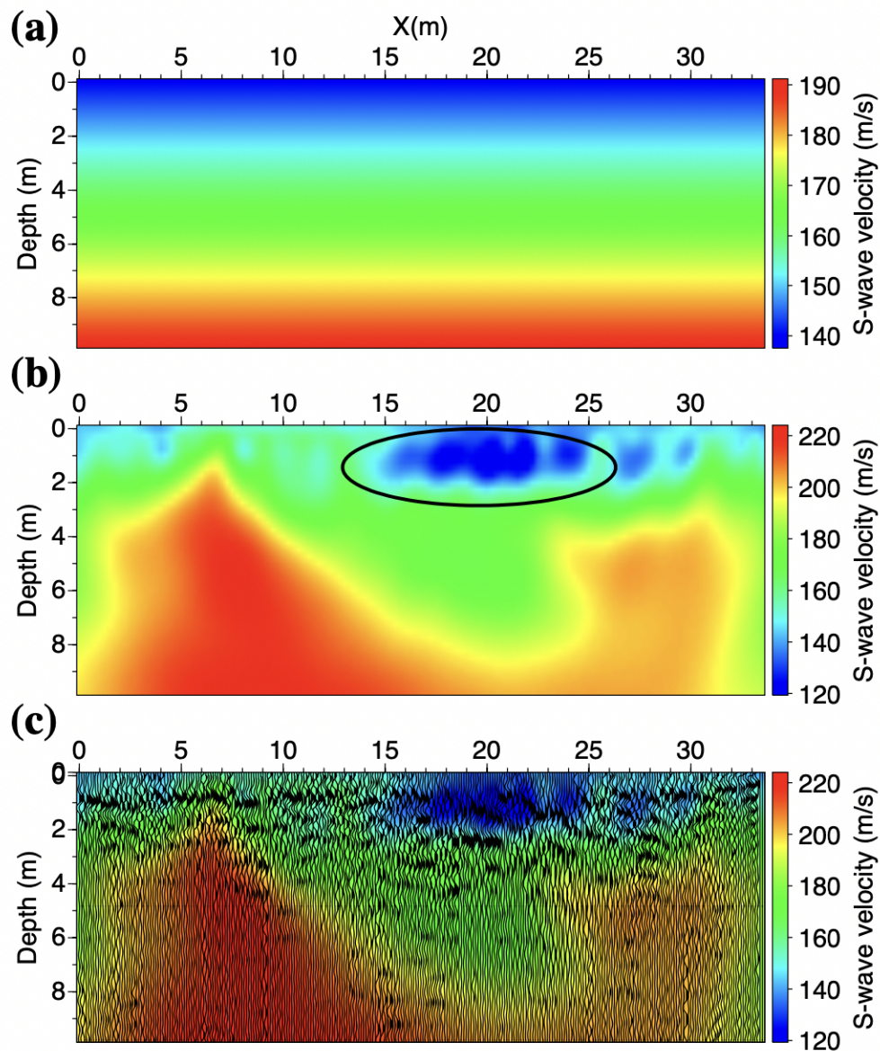
Figure 12: Inverted V_S model for seismic line A. (a) Initial model used in inversion; (b) result of instantaneous-phase coherency FWI after the 6th stage of sequential inversion (i.e., frequency band 5 \sim 60 Hz); (c) the overlay of CMP stacked section from S-wave reflection data (Ghose, 2020) and the inverted V_S model shown in (b). The ellipse in (b) marks the area where a tumulus was previously identified
