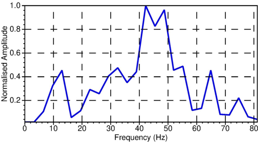
Figure 11: Average amplitude spectrum of 37 preprocessed shot gathers acquired along with seismic line A. 81x51mm (300 x 300 DPI)
