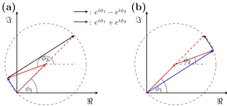
Figure 01: Illustrations of instantaneous-phase coherency as defined in equation 7. The red arrows denotes e^{i\phi_1} and e^{i\phi_2} , whereas the black and blue arrows represent e^{i\phi_1} - e^{i\phi_2} and e^{i\phi_1} + e^{i\phi_2} , respectively. The black arrow measures how the instantaneous phases of two signals are close to each other, while the blue arrow measures how much the instantaneous phases of two signals differ from 180 degrees. Either of the two measurements can be used on its own as a misfit function of FWI by matching the instantaneous phase between the measured and the synthetic data. Using numerical experiments (not shown in this paper), we found that the performance of different misfit functions (black arrow, blue arrow, combination of black and blue arrows) is quite similar. The reason why we design a misfit function with a combination of black and blue arrows is that this approach is novel and it has the chance to be more robust to noise. J(t) is obtained by subtracting the square of the two vectors given by the black and the blue arrows. (a) When the two signals have significantly different instantaneous phases, J(t) will be close to 1. (b) When the two signals have similar instantaneous phases, J(t) will be close to -1.
