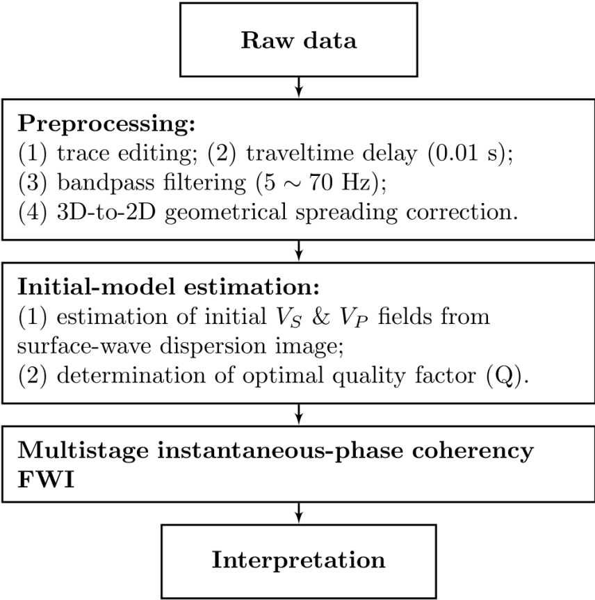
Figure 09: Workflow for field-data application of the instantaneous-phase coherency FWI.
