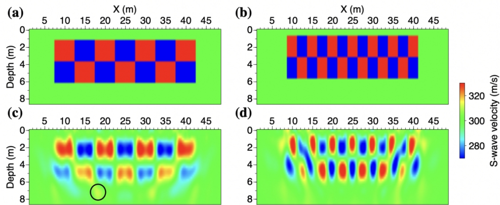
Figure 03: Checkerboard tests for resolution analysis. (a) True V_S model containing velocity anomalies. The size of these anomalies is 5 \times 2.5 \text{ m}^2 ; (c) the result of instantaneous-phase coherency FWI. (b), (d) the same as in (a), (c) but for anomalies with size of 2.5 \times 2.5 \text{ m}^2 . A homogeneous background ( V_S = 300 \text{ m/s} ) is used in all tests. The black circle indicates an artifact caused by the FWI algorithm.
