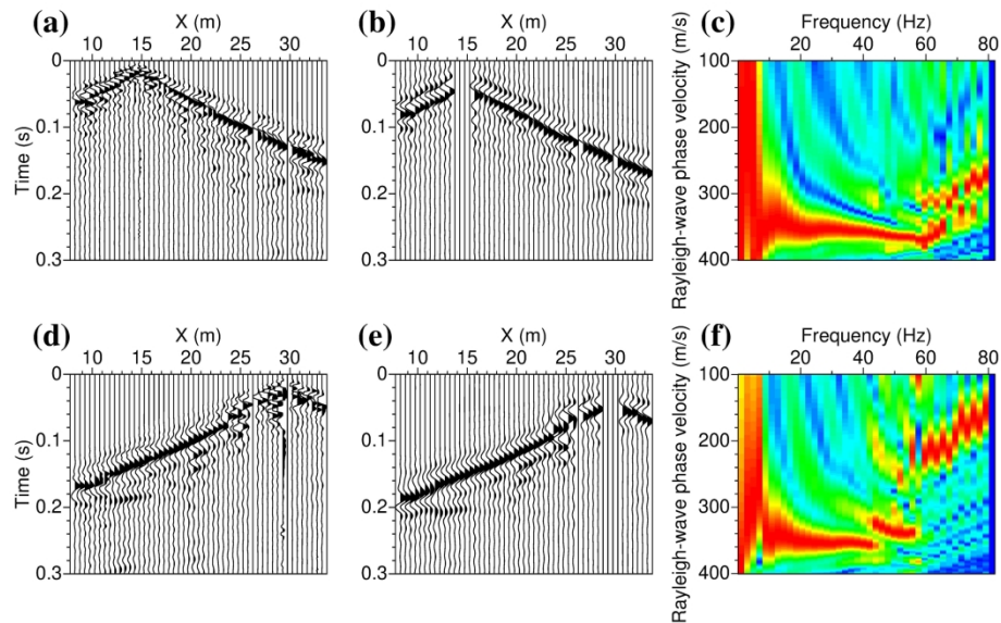
Figure 10: (a) Muted common-source gather along with seismic line A, where the source is positioned at x = 14.5 m; (b) the same as (a) but after preprocessing described in the text; (c) Rayleigh-wave dispersion image obtained by slant-stacking of the preprocessed shot gather shown in (b). (d), (e), (f) are respectively same as (a), (b), (c) but for a common-source gather where the source located at x = 29.5 m.
