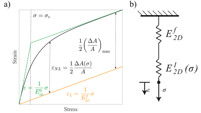
FIG. 1. Phenomenological model of the effective stress-strain response of biaxially tensioned wrinkled graphene membranes. (a) Schematic representation of the bilinear approximation and its independent and dependent parameters. The solid black line is the response of a wrinkled membrane following Eqs. (1)–(3), the solid orange line represents a pristine unwrinkled membrane and the dashed-dotted green lines are the tangents to the curve close to the origin and at maximum stress [bilinear approximation, Eq. (4)]; (b) spring-in-series system with a linear spring with constant stiffness representing the intrinsic stiffness of flat pristine graphene E_{2D}^f and nonlinear spring with a stress-dependent stiffness E_{2D}^I(\sigma) representing the stiffness of the wrinkles.
