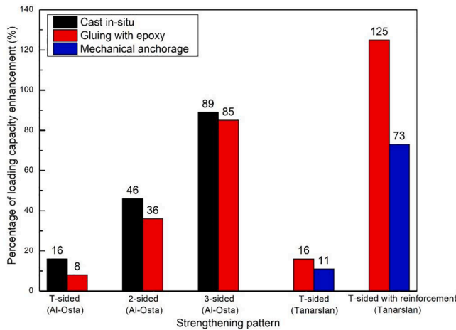
Fig. 16. Loading capacity enhancement with different bonding techniques (calculated as (F_{u,s}/F_{u,c} - 1) \times 100\% , F_{u,s} is peak load of strengthened beam, F_{u,c} is peak load of control beam) [77,107].
