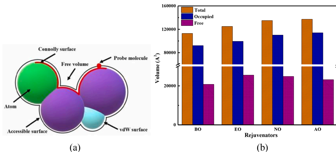
Fig.11. The volumetric parameters of different rejuvenators at 298 K.
