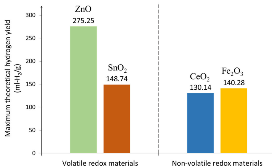
Figure 10. Comparison of the maximum theoretical hydrogen yields under standard conditions, calculated based on the redox limits for the volatile redox materials \text{ZnO} and \text{SnO}_2 and the non-volatile redox materials \text{CeO}_2 and \text{Fe}_2\text{O}_3 . Redrawn from [38].
