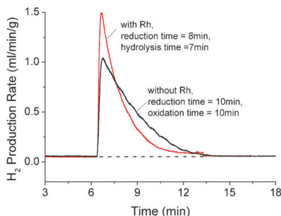
Figure 14. Effects of rhodium added to cerium (IV) oxide on the reduction and oxidation times, as well as on the hydrogen production rate during isothermal cycling at a temperature of 1500^\circ\text{C} . Reprinted from [64].
