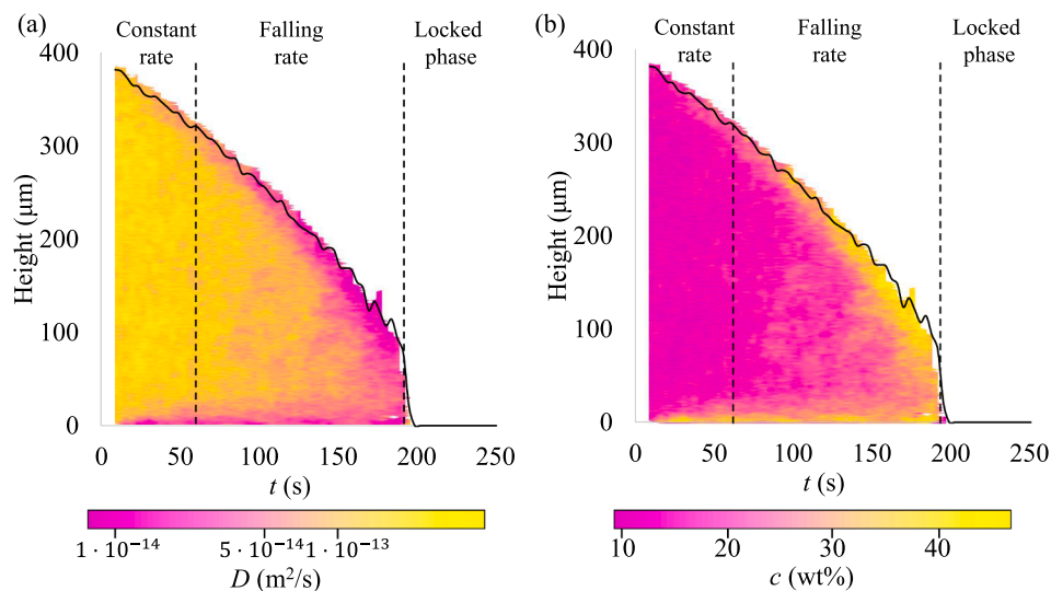
Fig. 5. Mapping of the intra-droplet properties. (a) Local logarithmic diffusion coefficient of the \text{TiO}_2 particles. (b) Local MD12 concentration. In both figures, the black line indicates the height of the droplet, as determined from the 1D OCT scans. The dashed lines indicate the transition between the different drying regimes.
