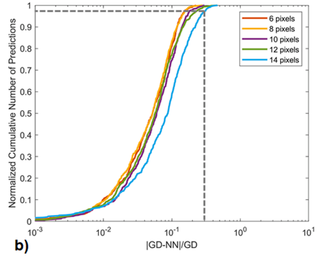
Fig. 6. Cumulative number of predictions as a function of the predictions' deviation from simulation results. Results along the x-direction (a) and the y-direction (b).
