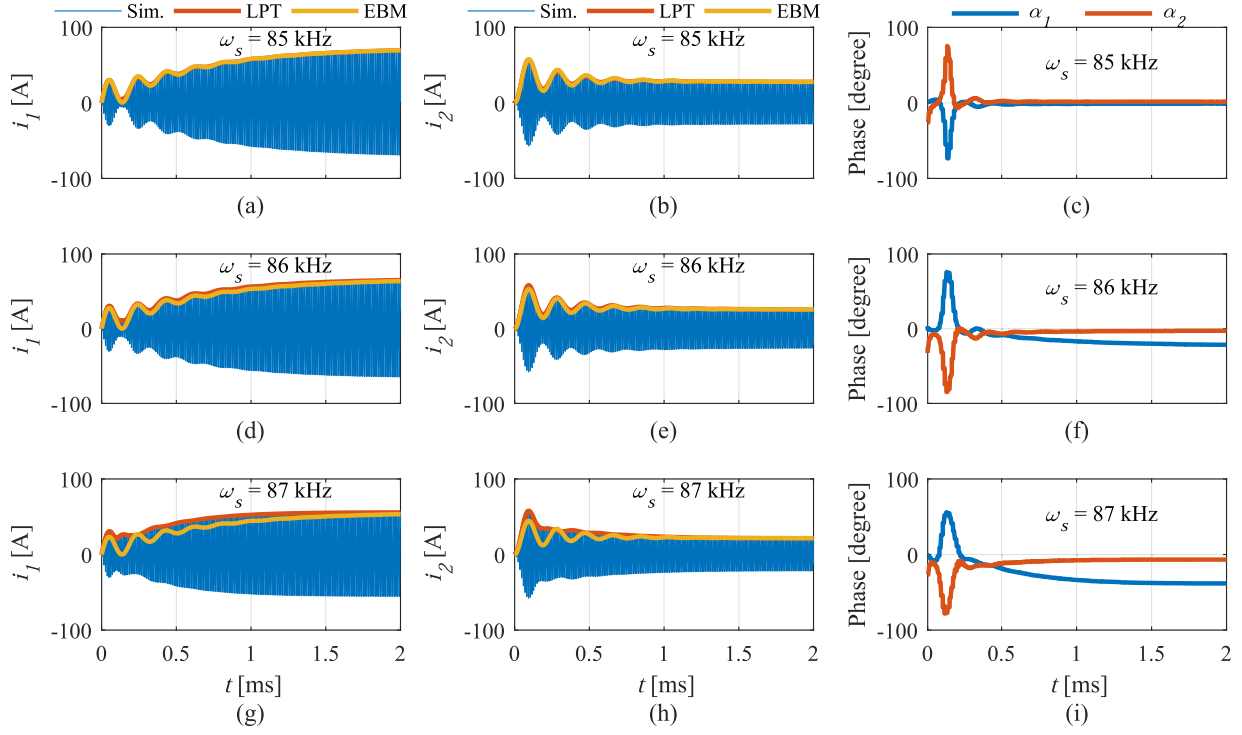
Fig. 7. Comparison between dynamic models using EBM and circuit simulations, where u_{in} = 100 V, \omega_r = 85 kHz, and C_{fo} = 80 \mu F, and the rest of the circuit parameters are the same as Fig. 4.
