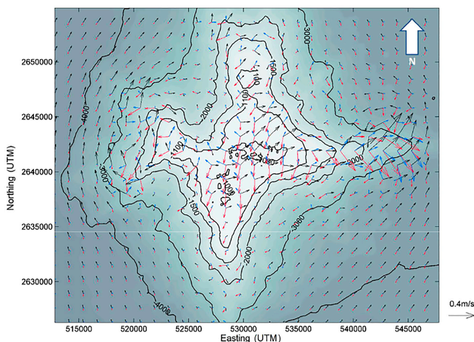
FIGURE 3 | Snapshots of currents 10 m above the bed in the vicinity of the Tropic Seamount, during a spring tide at HW (black), HW+4 h (ref) and HW+8 h (blue) (Spearman et al., 2020).
