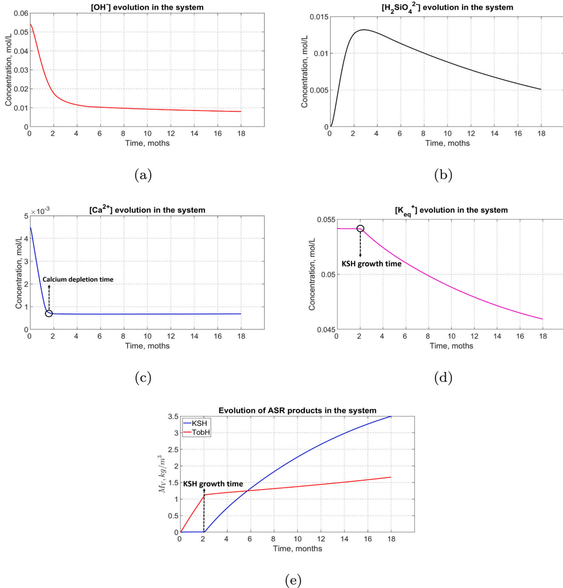
Fig. 3. The concentration evolution of \text{OH}^- (a), \text{H}_2\text{SiO}_4^{2-} (b), \text{Ca}^{2+} (c) and K_{\text{eq}}^+ (d) in system S_{15} within 540 days; (e): Mass evolution of KSH and TobH represented by M_V in system S_{15} within 540 days.
