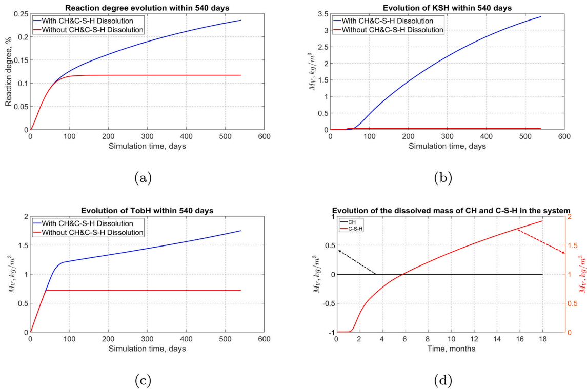
Fig. 8. (a): The reaction degree (the dissolved silica divided by the total mass of silica in the aggregate) evolution in system S 15 with or without CH and C-S-H dissolution within 540 days; (b) and (c): Mass evolution of KSH (b), TobH (c) represented by M_V in system S 15 with or without CH and C-S-H dissolution within 540 days; TobH (d): Mass evolution of dissolved CH and C-S-H represented by M_V in system S 15 within 540 days.
