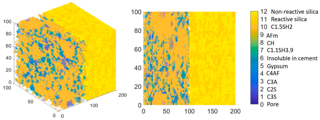
Fig. 1. A schematic diagram of the 3D domain of interest in the model and a 2D slice from the 3D domain. The left cube is cement paste and the right cube is aggregate. Different color represents different phases. unit of scale: \mu\text{m} .
