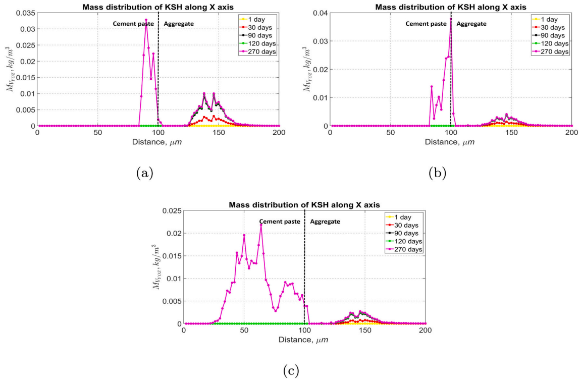
Fig. 11. The mass distribution evolution of KSH along X axis represented by M_{KSH} in systems with different alkali concentrations in the cement paste within 270 days. (a): in system S_{11} with 0.20 \text{ mol} \cdot \text{L}^{-1} alkali concentration; (b): in system A_{11} with 0.38 \text{ mol} \cdot \text{L}^{-1} alkali concentration; (c): in system A_{21} with 0.50 \text{ mol} \cdot \text{L}^{-1} alkali concentration.
