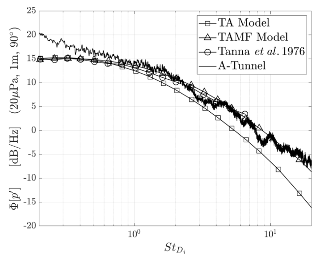
Fig. 13 Spectral density of the acoustic pressure fluctuations at 90^\circ from the jet axis. All results are scaled to the case of M_j = 0.15 , temperature ratio T_j/T_\infty = 1 and far-field location r/D_j = 20 : microphone results from this study (A-tunnel), experimental results from Tanna et al. (1976), prediction values from Tam and Aurialt (1999) original model (TA), and with empirical coefficient modified to the experimental data as in Morris and Farassat (2002) (TAMF)
