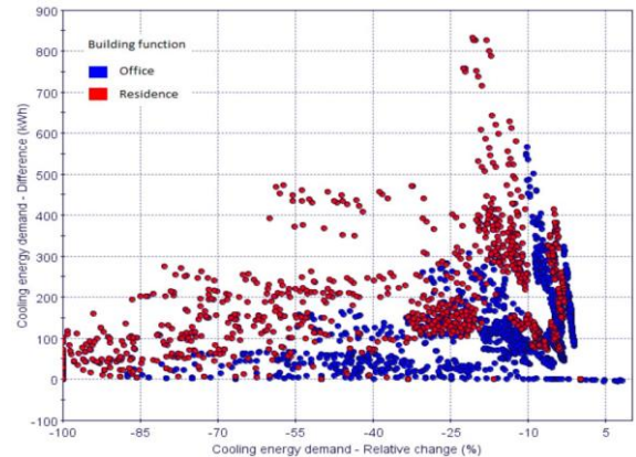
Fig. 7b – Difference in cooling demand (absolute and relative) between room without and with Trombe wall for offices versus houses [13]. Positive absolute values / negative percentages denote that the Trombe wall leads to an energy saving.
