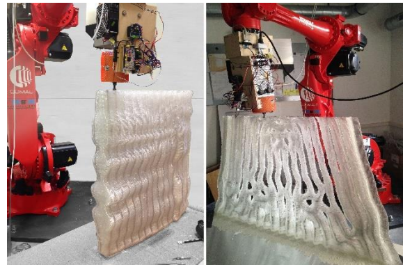
Fig. 12 – Robotically 3D printing of the prototype of the developed PCM based Trombe wall.
