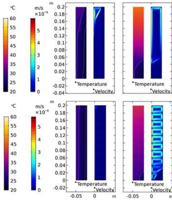
Fig. 9 – Temperature and fluid flow inside a block of PCM with a melting temperature of 25 °C and a thickness of 30 mm exposed to a radiation source of 300 W·m -2 , after exposure of 4 (left) and 8 hours (right). The top image shows an unsegmented block of PCM; the bottom image shows a segmented block of PCM (2 cm). [15]
