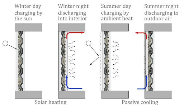
Fig. 1 - Principle of the latent heat storage unit [11].
