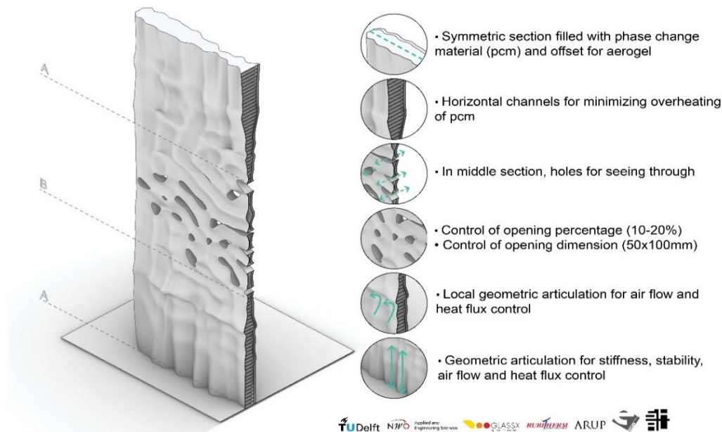
Fig. 14 – Final design of the prototype of the Double Face 2.0 PCM-based rotatable Trombe wall.
