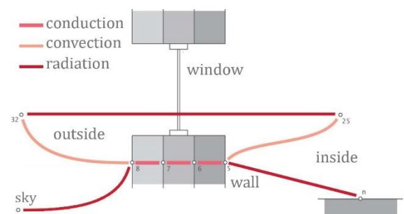
Fig. 3a - Heat transfer between nodes near window without Trombe wall [12].
