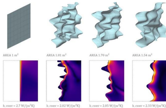
Fig. 11 – Effect of surface geometry on convective heat transfer coefficient [17].
