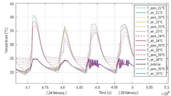
Fig. 10b – Temperature of the PCM and room air of an office space of 60 m 2 for different PCM melting temperature (mid-point of range at 20 to 26 °C with \Delta T of 3 °C) under sunny winter conditions using NEN5060 weather data [11].
