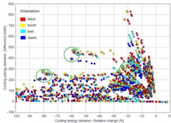
Fig. 8b – Difference in cooling demand (absolute and relative) between room without and with Trombe wall for different orientations [13]. Positive absolute values / negative percentages denote that the Trombe wall leads to an energy saving. The green circles denote how certain cases change if their orientation changes.
