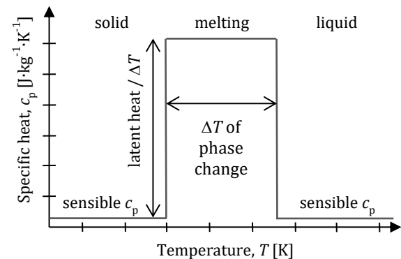
Fig. 2 - Modelling of the latent heat as part of the specific heat capacity.
