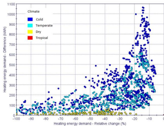
Fig. 6a – Difference in heating demand (absolute and relative) between room without and with Trombe wall for different climates [13]. Positive absolute values / negative percentages denote that the Trombe wall leads to an energy saving.
