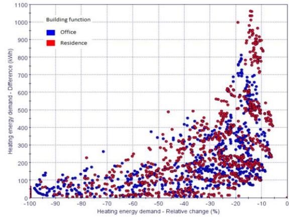
Fig. 7a – Difference in heating demand (absolute and relative) between room without and with Trombe wall for offices versus houses [13]. Positive absolute values / negative percentages denote that the Trombe wall leads to an energy saving.
