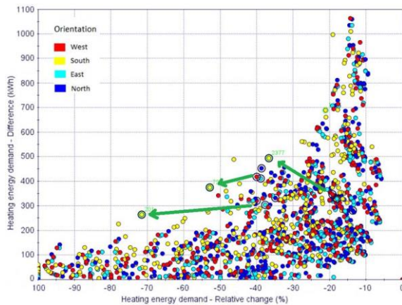
Fig. 8a – Difference in heating demand (absolute and relative) between room without and with Trombe wall for different orientations [13]. Positive absolute values / negative percentages denote that the Trombe wall leads to an energy saving. The green arrows denote how certain cases change if their orientation changes.
