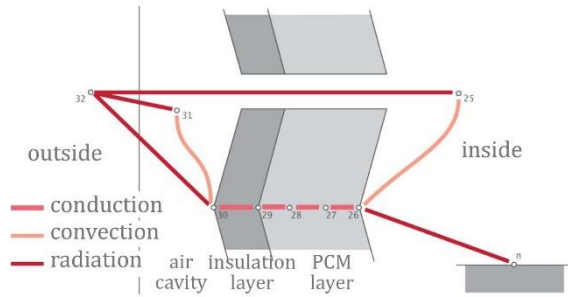
Fig. 3b – Heat transfer between nodes near window with Trombe wall [12].
