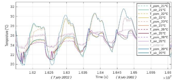
Fig. 10a – Temperature of the PCM and room air of an office space of 60 m 2 for different PCM melting temperature (mid-point of range at 20 to 26 °C with \Delta T of 3 °C) under warm summer conditions using NEN5060 weather data [11].
