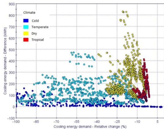
Fig. 6b – Difference in cooling demand (absolute and relative) between room without and with Trombe wall for different climates [13]. Positive absolute values / negative percentages denote that the Trombe wall leads to an energy saving.
