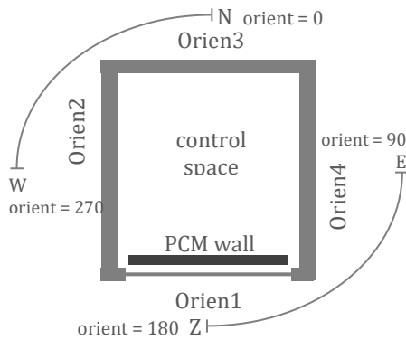
Fig. 4 – Floor plan model of the simulated room. The orientation may vary in the model.
