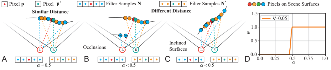
Fig. 6. A: The left filter samples (N) and the right filter samples (N*) of pixel p have similar distance to P . B-C: Due to occlusions or inclined surfaces, (N) and (N*) have different distance to P . D: Plots of the weight w used when combining filtered values from each view.
