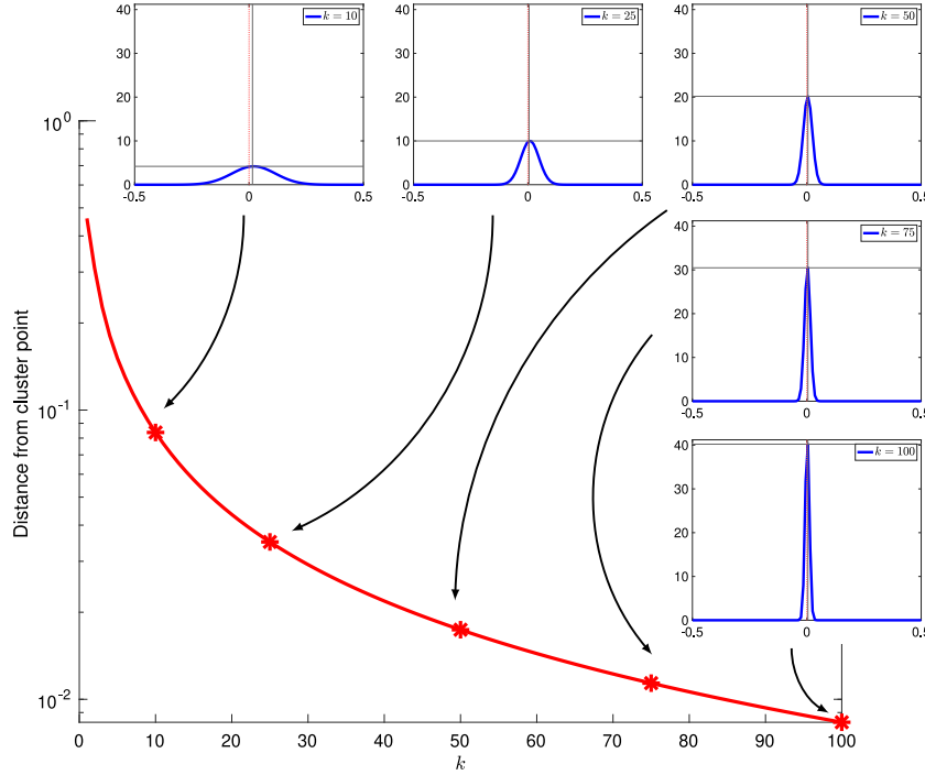
Fig. 6. The big plot shows how the average distance from a cluster point of the sequence \mathbb{E}[v^{k+1} | \mathcal{F}_k] = (1 + \delta^k)v^k + \epsilon^k - \theta^k , generated by Robbins–Siegmund Lemma (Lemma 4.1), goes to zero as the number of iterations increases. The small plots show how the distribution of the distance from a cluster point varies with the iteration toward a probability distribution centered at 0, i.e., the sequence converges a.s.
