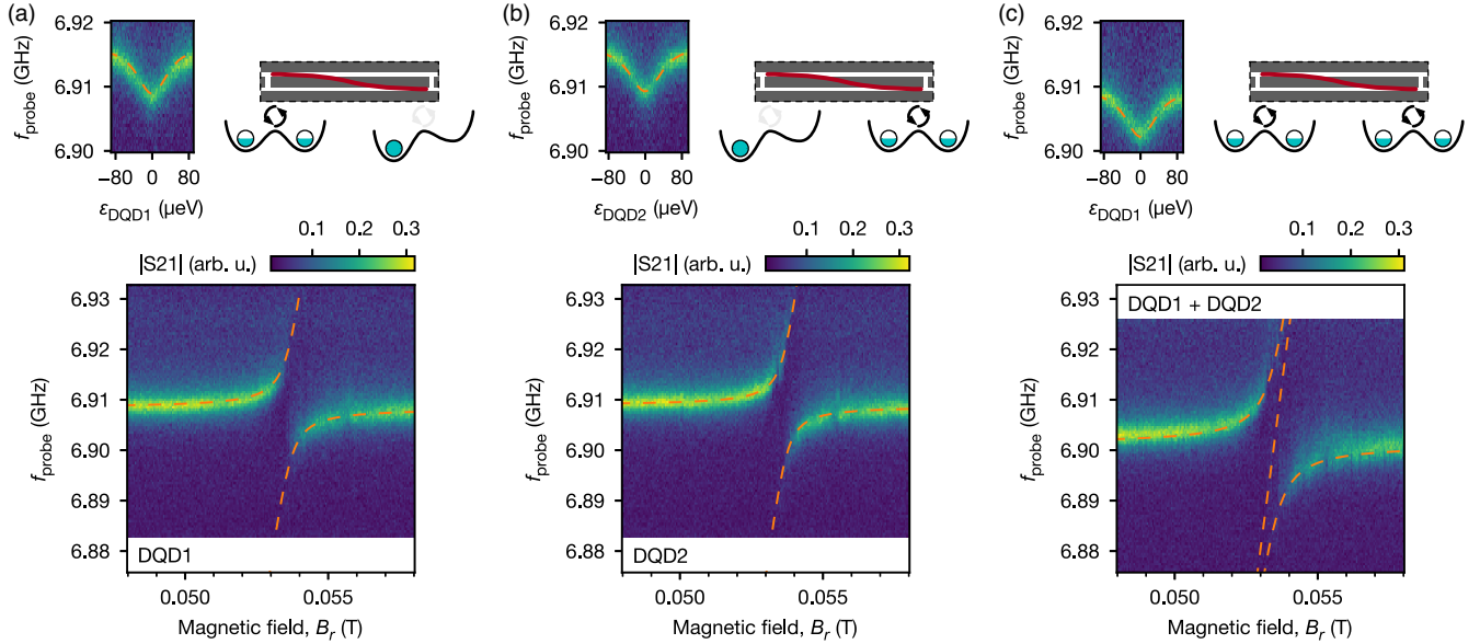
FIG. 2. Resonant spin-photon-spin coupling. (a,b) Spin-photon vacuum Rabi splitting of DQD1 (a) and DQD2 (b) for tunnel splittings (2t_c^1, 2t_c^2)/h = (13.2, 13.7) GHz and a field angle of \phi = 10.5^\circ . When the gate voltage is set on the zero-charge-detuning point, which corresponds to the middle of the (0,1)-(1,0) interdot charge transition, the charge-photon interaction g_c/2\pi = 192 MHz between the DQD charge and the resonator dispersively shifts the resonator frequency (insets) and enables the spin-photon interaction through the artificial spin-orbit interaction. The dashed lines are the Hamiltonian model transitions. The probe power is -117.5 dBm. (c) When both dots interact simultaneously with the resonator, the dispersive shifts are additive, and the vacuum Rabi splitting is enhanced by a factor of approximately \sqrt{2} , an effect of the coherent collective spin-photon interaction. Model transitions are adjusted to the individual interaction data and used to predict the simultaneous interaction data.
