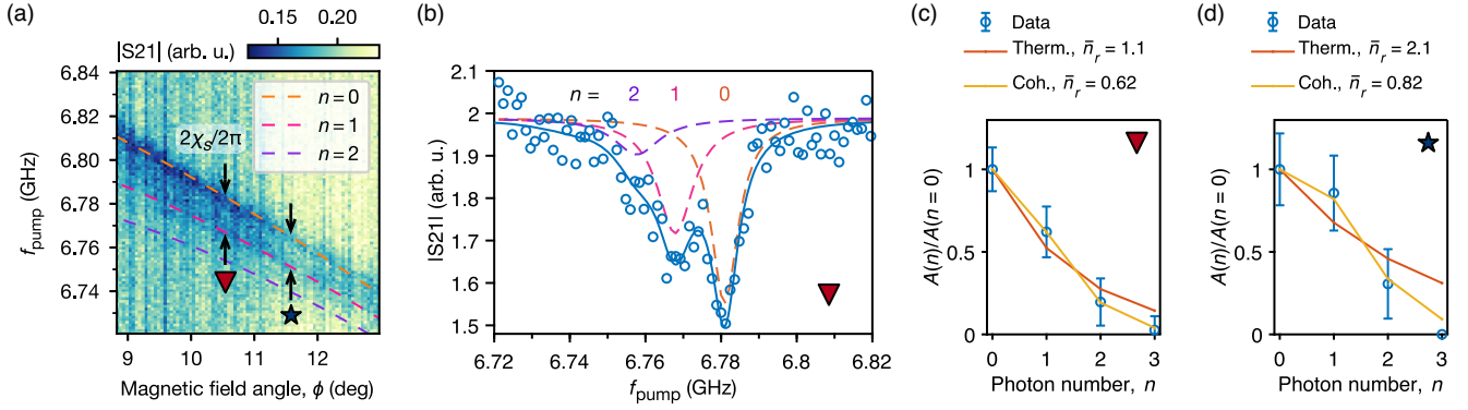
FIG. 4. Photon-number-resolved spin dispersive shift. (a) Spin transition frequency of DQD1 showing an extra dip below the main transition for larger probe power. The dip matches well the prediction from the Hamiltonian model (dashed lines) for |\downarrow, n\rangle \leftrightarrow |\uparrow, n\rangle transitions, with the first two transitions visible in this plot. (b) Line cut of the data in panel (a) for \phi = 10.55^\circ , and fit to four Lorentzian dips (first three shown with dashed lines). A dispersive shift 2\chi_s/2\pi = -13.1 \pm 2.2 MHz is extracted. (c) Relative area of the dips for \phi = 10.55^\circ , and comparison with thermal [ P_{\text{thermal}}(n) = \bar{n}_r^n / (\bar{n}_r + 1)^{n+1} ] and coherent [ P_{\text{coherent}}(n) = e^{-\bar{n}_r} \bar{n}_r^n / n! ] photon-number distributions. The error bar represents the 95% confidence interval. (d) Relative area for \phi = 11.6^\circ . At this angle, the resonator has a smaller \kappa'_r , resulting in a larger steady-state photon number. The coherent-state distribution has better agreement.
