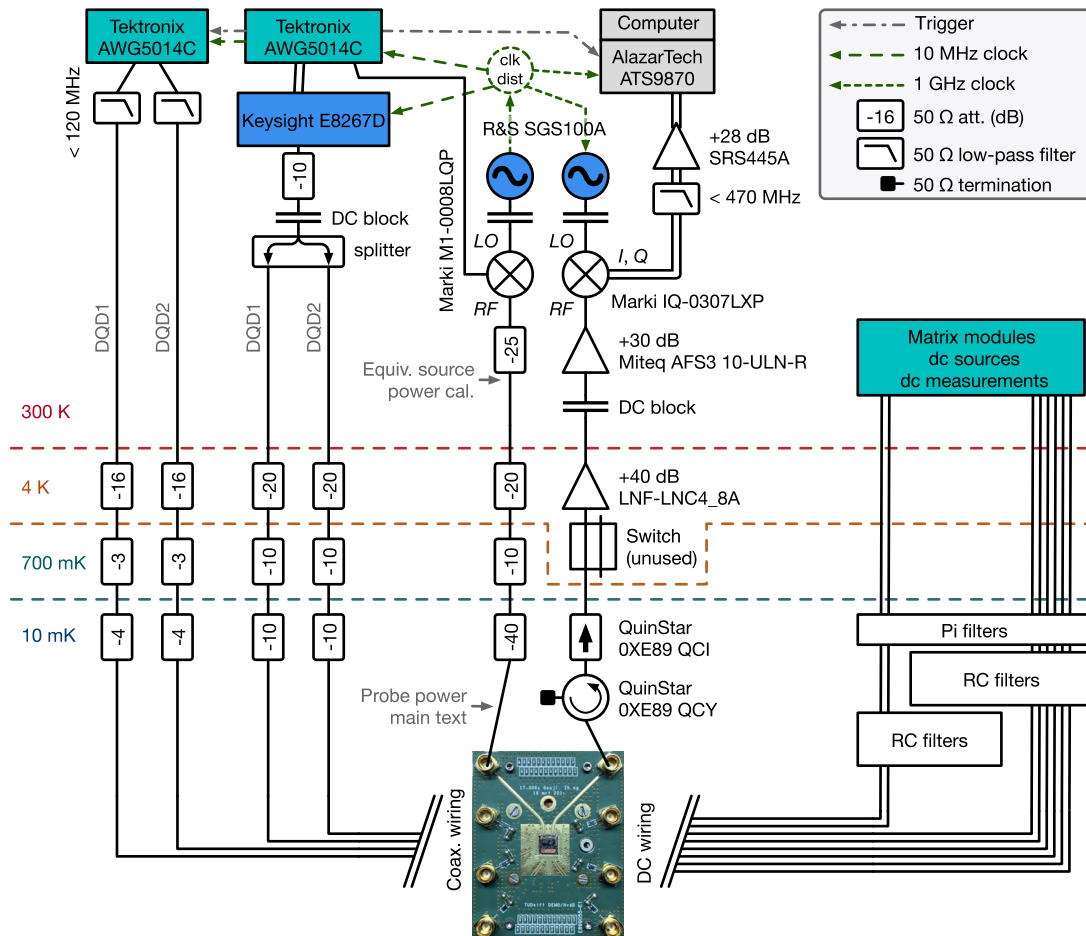
FIG. 6. Schematic of the measurement setup.
