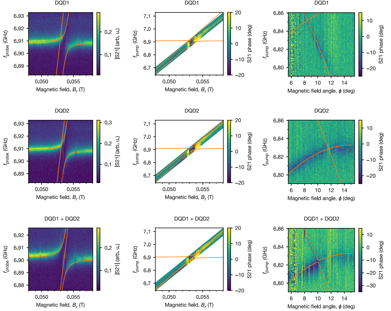
FIG. 9. Example of data used to extract model parameters. For this set, 2t_c/h = 13.5 GHz, B_r = 52 mT, and \phi = 10.5^\circ . The first column shows vacuum Rabi splitting reconstructions for individually and simultaneously interacting spins. The second column shows dispersive spin sensing (the data near spin-photon resonance are scrambled because of the close proximity of the levels). The third column shows the angular dependence of the spin levels with dispersive spin sensing. The two spinlike and the photonlike transitions are shown together. These data, and more, are used to calibrate the micromagnet parameters for use in the Hamiltonian model Eq. (D2). For these tunnel splittings and spin-photon detunings, the model predicts g_s/2\pi = 11.4 MHz and 2J/2\pi = 3.3 MHz. Here, 2J/2\pi is too small to be resolved. Note that transition linewidths are power broadened.
