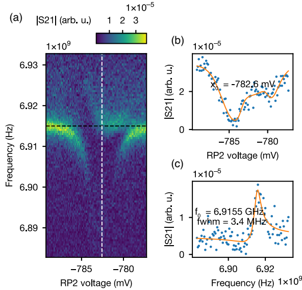
FIG. 7. Fitting of zero charge detuning. (a) Example of a single frame of data used in a vacuum Rabi splitting reconstruction. (b) Cut along the black line from panel (a) corresponding to the bare resonator frequency to extract the zero-detuning gate voltage x_0 . An empiric fitting function is used to find the center of the signal dip due to the dispersive shifts. (c) Cut along the fitted zero-detuning value x_0 (white line) and fit to a single Fano resonance.
