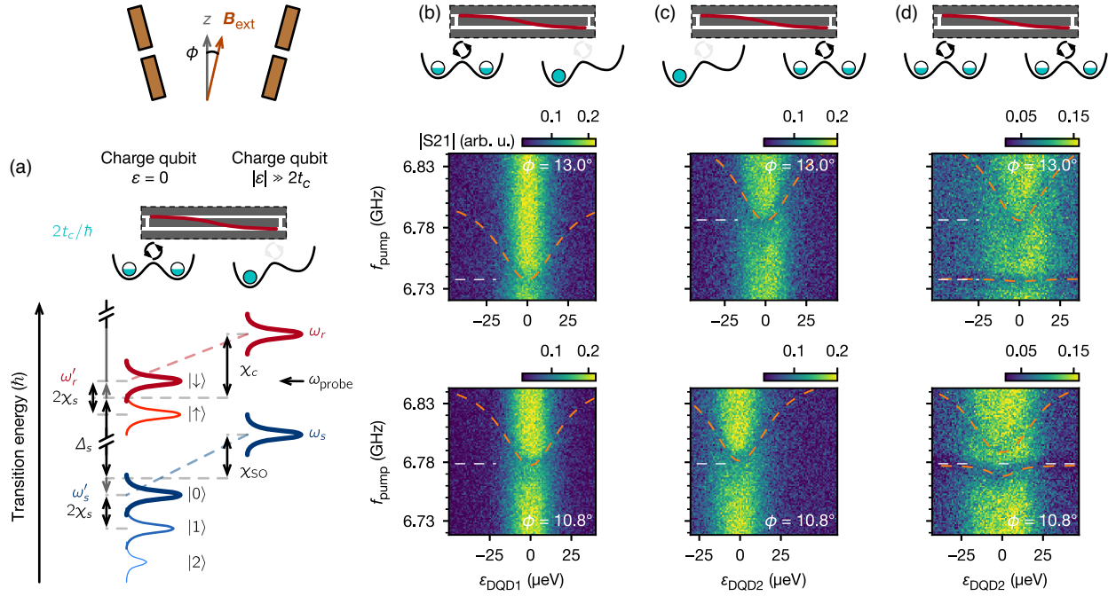
FIG. 8. Dispersive regime transitions, and spin-spin interaction versus DQD detuning. (a) Schematic representation of the transition energy shifts in the dispersive regime. See Appendix D for details. (b,c) Measurement of spin transitions for DQD1 (b) and DQD2 (c) as a function of the charge detuning \epsilon with dispersive readout, with 2t_c/h \approx 8.7 GHz and B_r = 52 mT. A pump tone is sent down the gate lines to excite the spins, resulting in a signal dip when the pump and spin frequencies match. Here, (f_{\text{probe}}^1, f_{\text{probe}}^2, f_{\text{probe}}^{12}) \approx (6.9038, 6.9061, 6.8981) GHz for \phi = 10.8^\circ . The spin transition frequency at \epsilon = 0 \mu\text{eV} is marked with a white dashed line for comparison between plots. (d) When the spins are simultaneously interacting with the resonator, the spin states hybridize depending on their energy difference. In the nonresonant case, \phi = 13.0^\circ , their energies are minimally perturbed, as can be seen by the model lines and the white guides. In the resonant case, \phi = 10.8^\circ , the two spins hybridize due to the exchange interaction 2J/2\pi = 20.2 MHz mediated by virtual resonator photons. The upper state is hardly visible because its symmetry makes it dark to the resonator probe, which is expected for a coherent spin-spin interaction.
