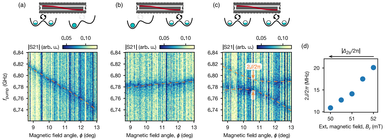
FIG. 3. Spin-spin coupling via virtual photons. (a,b) Dependence of the independently interacting spin transition frequencies as a function of the external magnetic field angle \phi at B_r = 52 mT. See Appendix C for the reconstruction procedure responsible for the vertical stripes. (c) When both spins interact simultaneously with the resonator, an avoided crossing is observed. The spin states hybridize with a splitting 2J/2\pi = 19.0 MHz, larger than any of the transition widths 2\Gamma_s/2\pi \leq (13.2 \pm 4.2) MHz. A dark state is observed along the upper branch, an effect caused by the symmetry of the coherently hybridized spin states. (d) Plot showing how the exchange interaction is reduced when the spin-photon detuning is increased.
