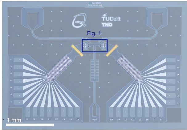
FIG. 5. Composite optical image of the device chip without wire bonds.
