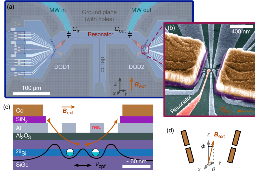
FIG. 1. Spin-spin coupling device. (a) Optical image of the resonator and QD areas with colored overlays. The ground plane, resonator, microwave (MW) in and out ports, and dc tap are thin superconducting NbTiN. The substantial kinetic inductance and resonator impedance result in a 6.916-GHz resonator that is only 250 \mu\text{m} long. (b) Colorized angled scanning electron microscope image of a (nominally identical) DQD gate structure and micromagnets. The NbTiN resonator end is contacted with an Al plunger electrode of the DQD, which is biased through the dc tap. (Image rotated 90^\circ .) (c) Schematic of the DQD heterostructure and gate stack using the same color scheme as in panel (b). A photon couples to an electron spin through spin-orbit (micromagnet) and orbital-photon (voltage zero-point fluctuations V_{\text{zpf}} ) interactions. (d) Micromagnets are tilted \pm 15^\circ , allowing one to fine-tune each spin's Zeeman energy through the external magnetic field angle \phi . Here, \mathbf{B}_{\text{ext}} = (B_r, \theta = -90^\circ, \phi) .
