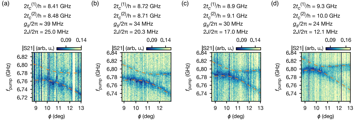
FIG. 11. Extended spin-spin hybridization data versus spin-photon coupling strength. (a)–(d) Dispersive spin-spin hybridization measured for decreasing spin-photon coupling values. The g_s is adjusted through its dependence on t_c and is approximately the same for both spins, while B_r = 52 mT is fixed. The \Delta_{2s}/2\pi \approx 78 MHz is approximately unchanged between plots because changes in \chi_{SO} are approximately compensated by changes in \chi_c . The model fully captures the observed transition frequencies within plots and between the plots, and the only adjustment is the experimentally measured t_c . As expected, 2J/2\pi decreases as g_s/2\pi decreases.
