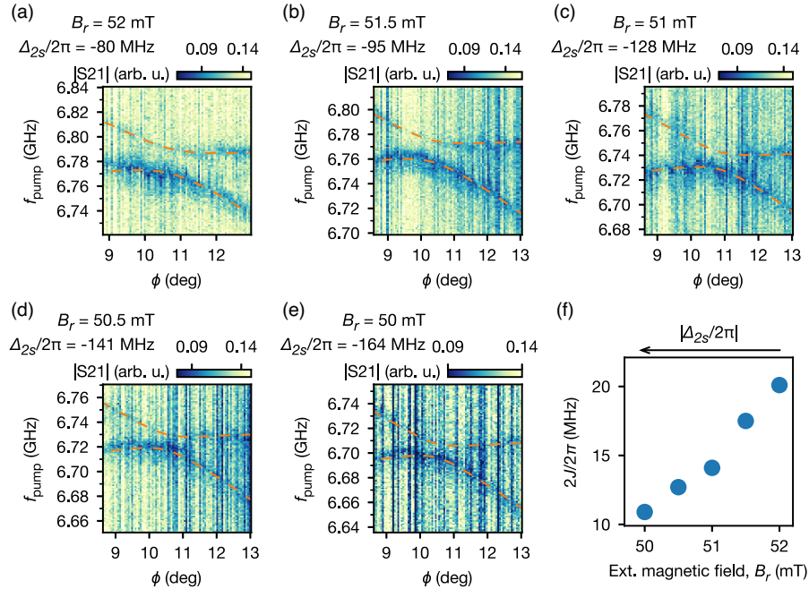
FIG. 10. Extended spin-spin hybridization data versus spin-photon detuning. (a)–(e) Dispersive spin-spin hybridization measured for different spin-photon detuning values. The probe power is larger for these data than for the data in Fig. 3; the shadow visible below the main transition is caused by the photon-induced dispersive shift of the spin. The apparent jitter of the transition energy as a function of \phi is caused by jitter of the DQD2 tunnel coupling over the time it takes to reconstruct all angles. The 2t_c/h \approx 8.7 GHz is retuned between plots and yields g_s/2\pi \approx 34 MHz for both spins. The model fully captures the observed transition frequencies within plots and between the plots, and the only adjustment is the experimentally measured small variations in t_c . (f) Splittings 2J/2\pi extracted from the model as a function of spin-photon detuning (through B_r ). Comparison with the linewidth is impaired by the photon-number broadening of the transitions. As expected, 2J/2\pi decreases as |\Delta_{2s}/2\pi| increases.
