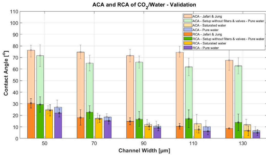
Fig. A.11. Advancing and receding contact angles (ACA and RCA) of \text{CO}_2 /water systems. The orange bars represent the results of Jafari and Jung (2017) using a similar chip at P = 10 bar and T = 21^\circ\text{C} . The green bars represent results of V1 with a setup similar to Jafari and Jung without filters and valves and with pure water, the yellow bars represent the results of V2 with water which was saturated with \text{CO}_2 and the purple bars represent the results of V3 with pure water. The error bars represent the standard deviation of the measurements.
