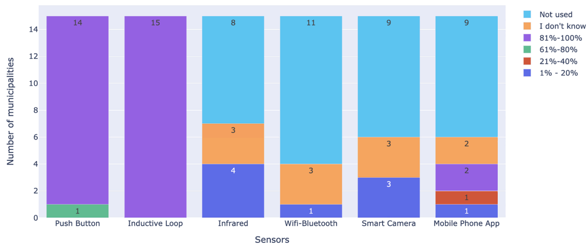
Fig. 4. Percentage of intersections equipped with the various kinds of bicycle sensors.
