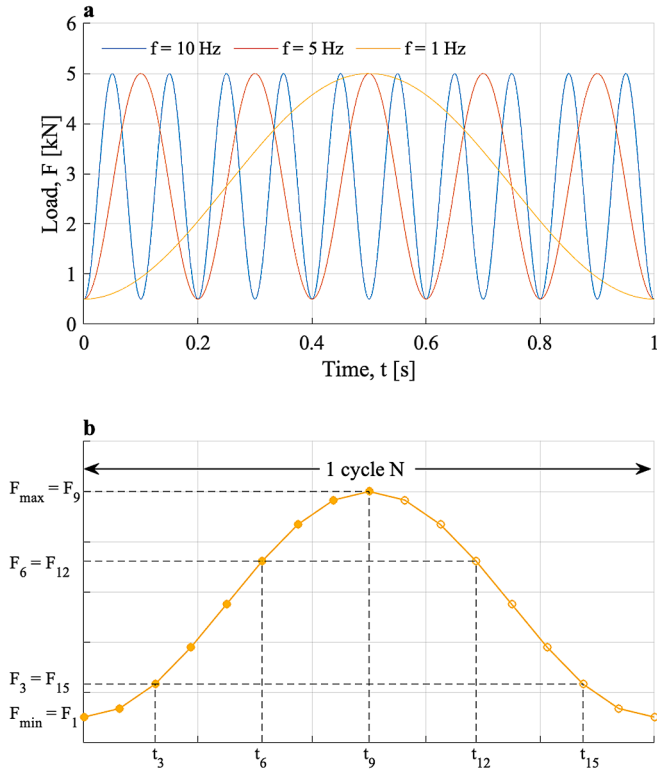
Fig. 10. (a) Load vs time for different loading frequencies; (b) Discretisation of the sinusoidal load F under frequency of f = 1 Hz by a time-step of dt = 0.0625 sec.
