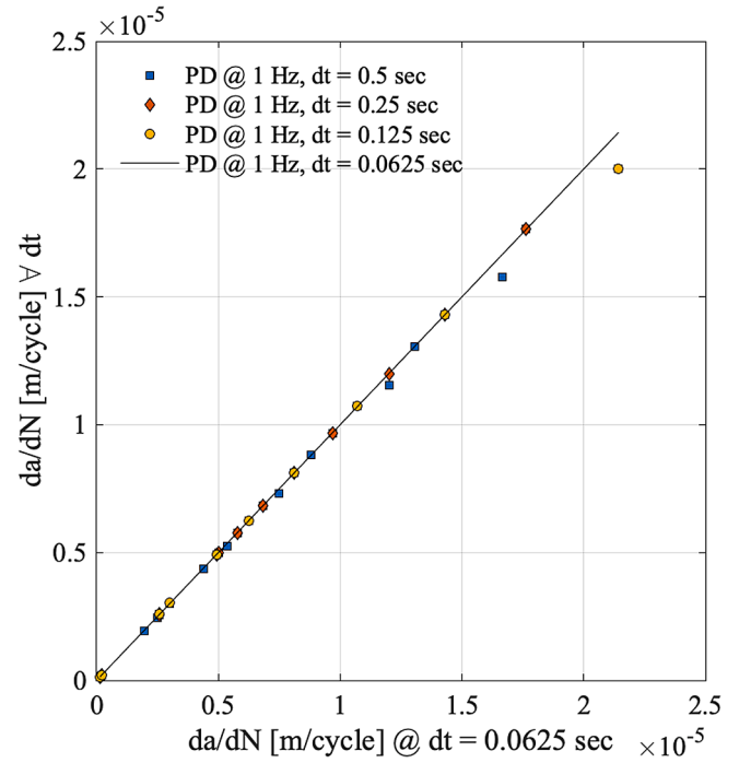
Fig. 11. Comparison between four different time-step sizes.
