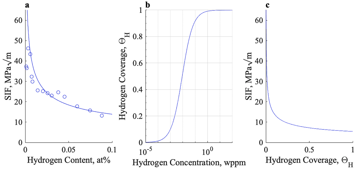
Fig. 3. a. Effect of Hydrogen content on the critical SIF, adapted from [41], b. Hydrogen Coverage, \theta_H as a function of Hydrogen Concentration [42] for \Delta G_b^0 = 40 \text{ kJ/mol} , c. SIF as a function of \theta_H .
