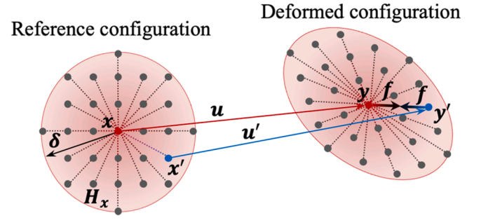
Fig. 2. Bond-based PD forces between two material points.
