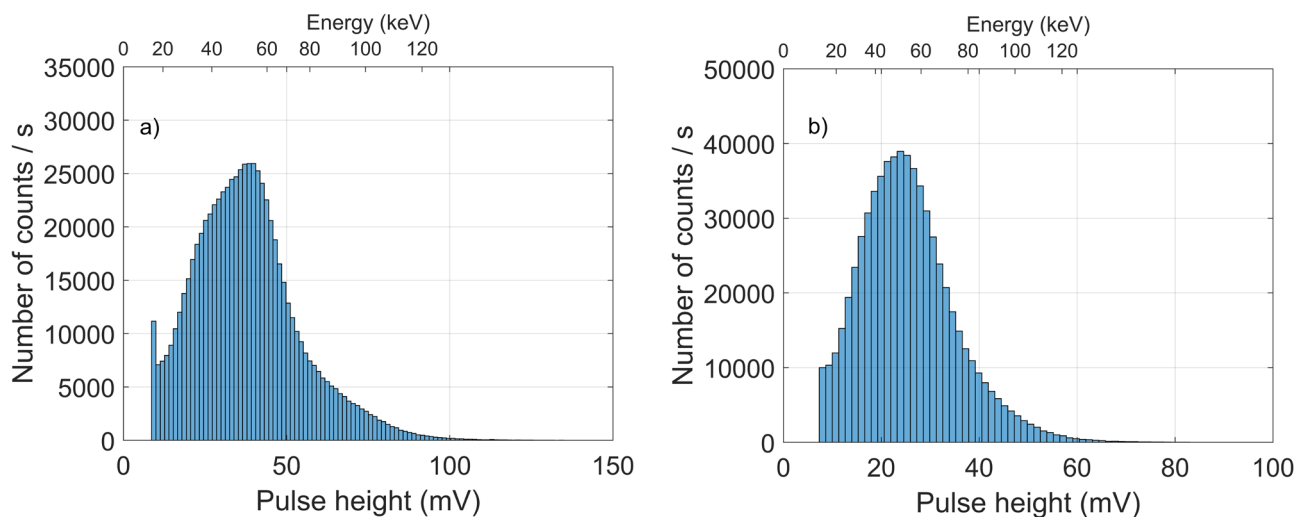
Figure 5. X-ray tube spectra (120 kVp, tungsten anode, anode angle of 20°, 3.0 mm Be and 7.5 mm Al filtration) measured using a) the LYSO and b) the YAP detector, for p-like counting with a 15 keV threshold at a tube current of 0.5 mA, i.e. under low fluence rate conditions. The energy-axes are based on the calibrations shown in figure 3b and figure 3c.
