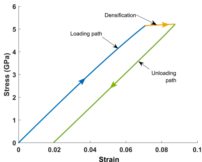
FIG. 8. Plot of stress–strain curve corresponding to experiment No. SSL-3. The uniaxial strain is also identical to the volumetric strain \left(1 - \frac{\rho_0}{\rho}\right) .
