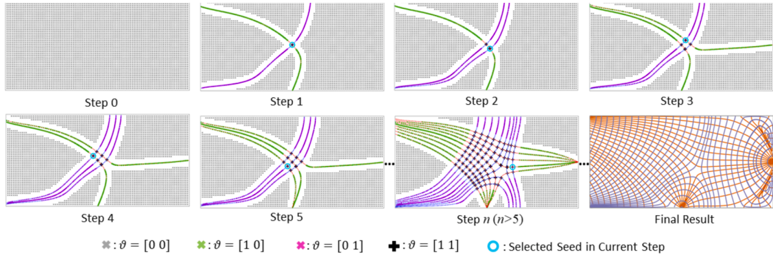
Fig. 2. Starting from a set of seeds with empty valence [0\ 0] , the sampling process is performed until all the seed valences have been turned to [1\ 1] . The other and blue lines are the major and minor PSLs. (For interpretation of the references to colour in this figure legend, the reader is referred to the web version of this article.)
