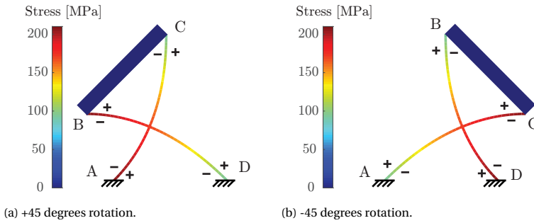
Figure 2.7: FEM simulations show the peak stresses of 210 MPa in the traditional CFP for large rotations.
