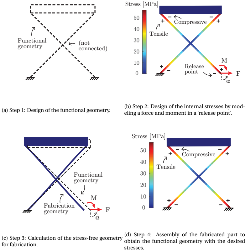
Figure 2.3: The four steps of the STAGE method, explained with the crossed-flexure pivot. The geometry in the last step is the same as in the first step and exhibits the desired stresses.
