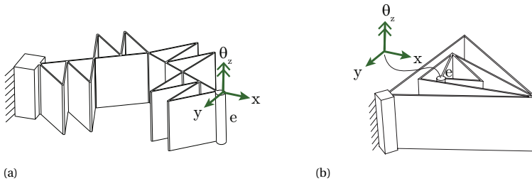
Figure 6.6: (a) 3-DoF planar joint 1, derived as special case from the Tetra I design in Fig. 6.2a; (b) 3-DoF planar joint 2, derived as special case from the Tetra II design in Fig. 6.5a.
