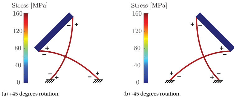
Figure 2.8: FEM simulations of the redesigned CFP showing peak stresses of 161 MPa, which is a reduction of 23 % compared to the traditional design. The fabrication geometry is shown in Fig. 2.3c.
