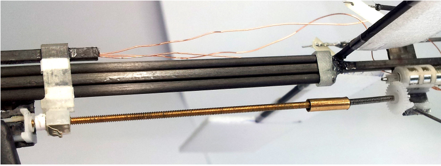
Figure 3.6: Two hard plastic injection molded sliders (white/left) clamp two round carbon rods (middle), over which the complete wing, motor house, motor, and Electronic Speed Controller (ESC) moves. The lead nut is attached to the main wing (bottom left). The lead screw runs via gearing to a small brushed motor (right)
