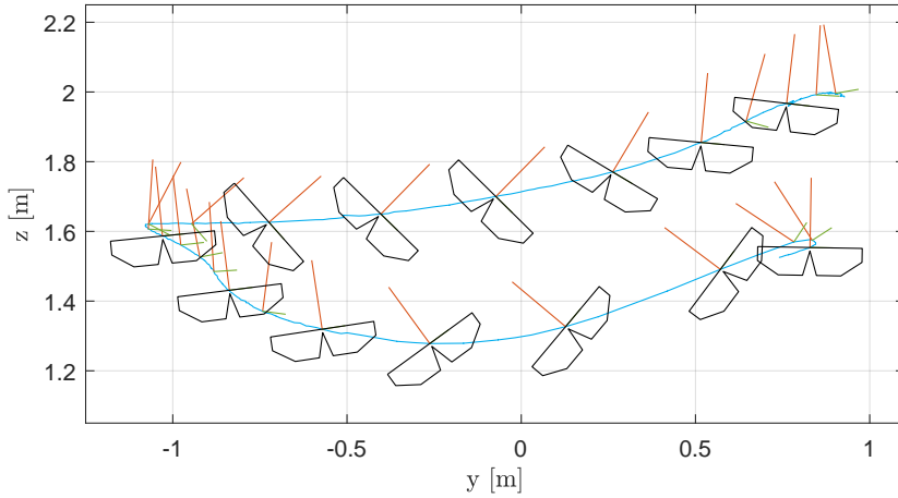
Figure 4.10: Indoor test flight recorded by the Optitrack motion tracking system. The quad-thopter starts at the bottom right and makes a 2 m step to the left and then back to the right in under 3 s. Notice that the vehicle does not need a negative roll angle during the slow down.
