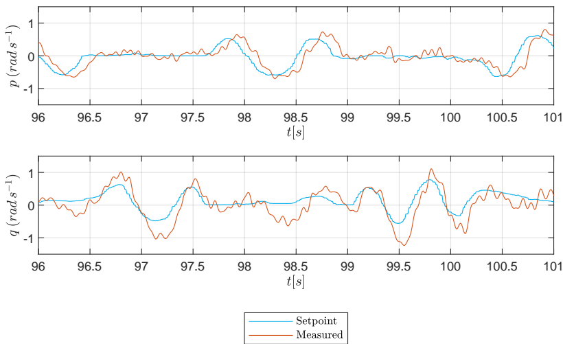
Figure 7.6: Performance test of an LQR controller derived directly from the identified TTP DelftaCopter model. The pilot manually commands the attitude rate of the DelftaCopter. The roll response has a small delay with the command but otherwise has adequate tracking performance. The pitch rate shows coupling with the roll and the response shows larger values than the command.
