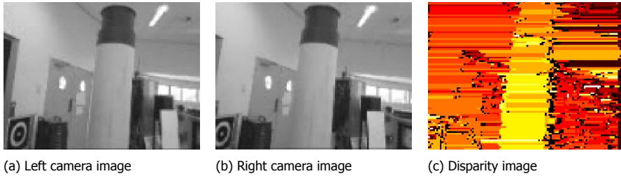
Figure 2.11: Sample disparity image if the 4g stereo vision system on 128 \times 96 pixels processed on a 168 MHz 32-bit DSP with a single camera port and only 196 kb of memory. In areas of low contrast, the algorithm propagates the disparity of the closest edge. While the disparity image is not state-of-the-art in terms of accuracy, in terms of memory and computational power, it nevertheless enables the 20 g robot to safely navigate.
