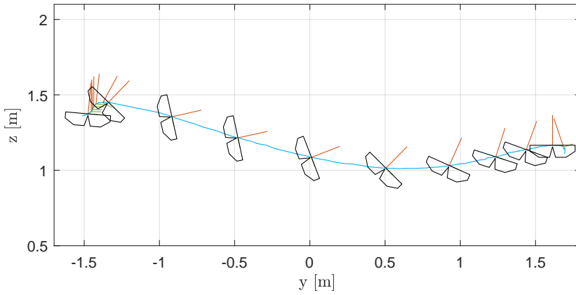
Figure 4.12: Lateral view of a manually flown 3m lateral step recorded indoors. The quad-thopter reaches a speed of 3.5 m/s and angles of 80° roll during this 1.5 s maneuver.
