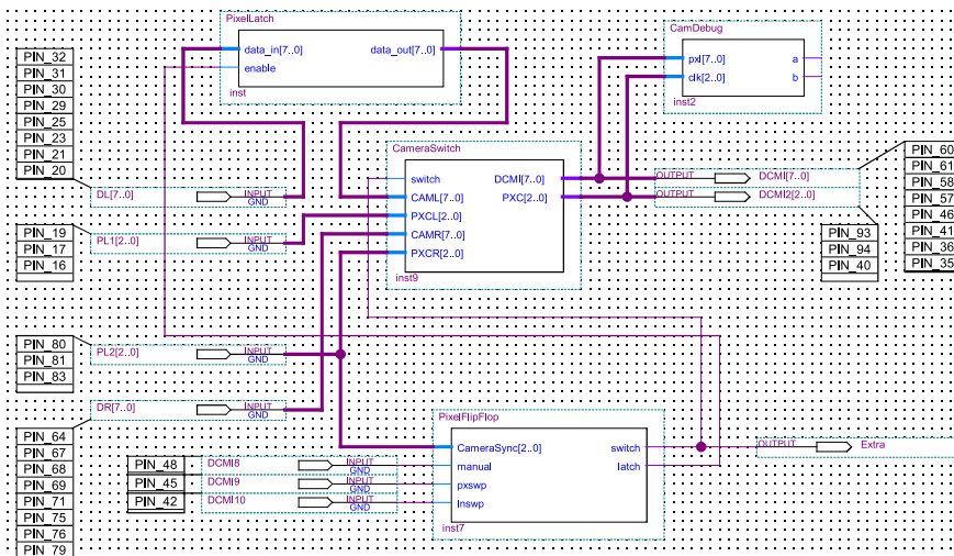
Figure 2.8: VHDL logic inside the stereo camera CPLD [7].
