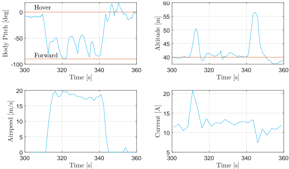
Figure 6.21: Close-up of a single transition. The DelftaCopter is starting from hover and transitions to forward flight. The current temporarily increases to over 20 A during the acceleration phase and altitude increases during this open-loop transition. It then flies a square pattern while the body pitch angle is used to control altitude. During each of the four turns, a significant pitch up is required to keep the altitude constant. Finally, the DelftaCopter transitions back to hover in a 3 s open-loop maneuver where all excess kinetic energy is transformed into altitude.
