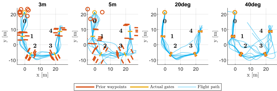
Figure 9.16: Robustness analysis in simulation on the Baltimore track with uniform flight plan gate position errors of 3m and 5m and uniform gate orientation errors of 20° and 40°. Perturbations in trajectories can be seen when the drone aligns with expected position of gates, but quickly have to correct after observing the real positions.
