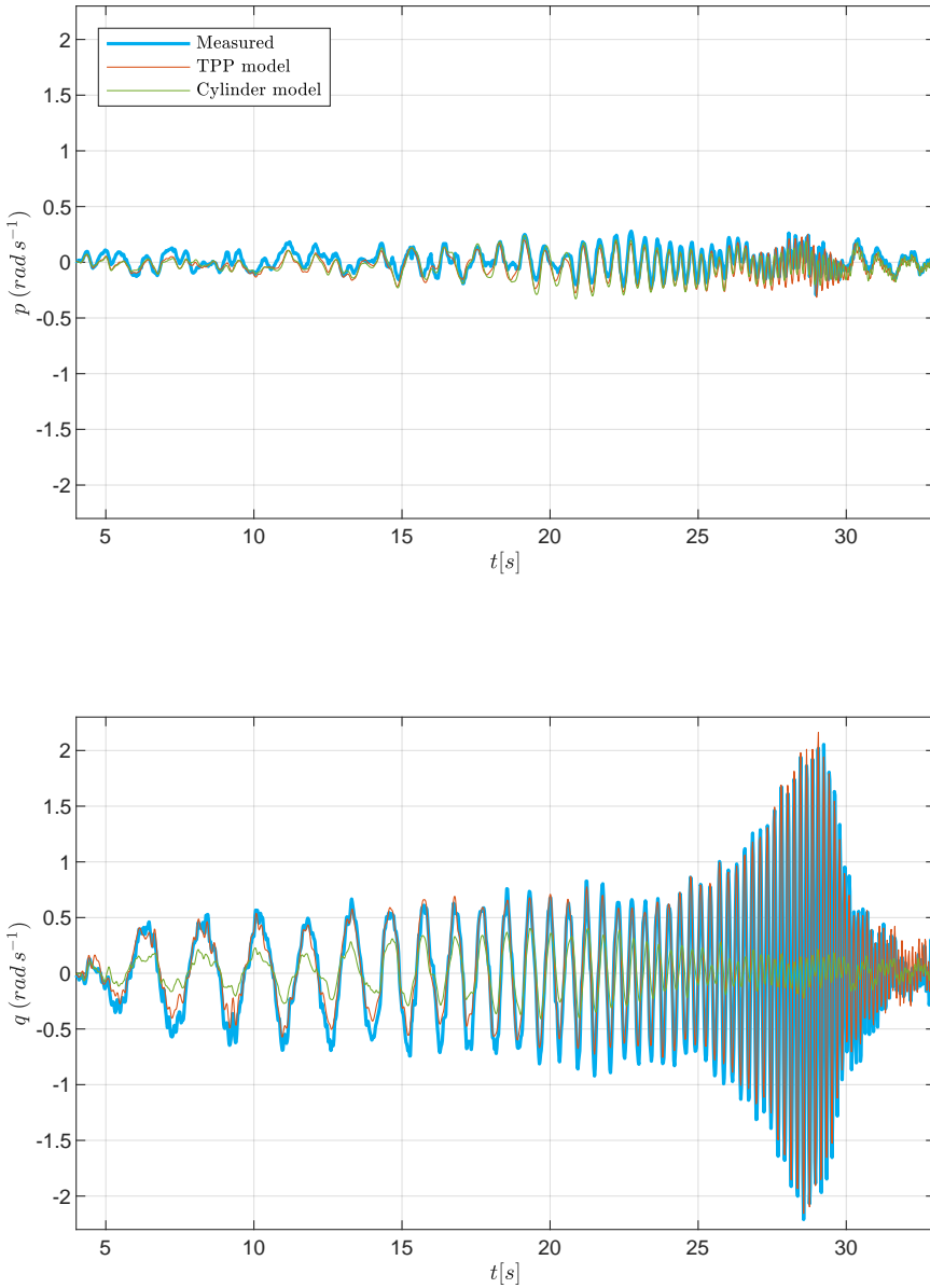
Figure 7.4: A chirp on the pitch axis in hover. The roll motion due to pitching is not as pronounced as the pitch due to roll since the roll inertia of the fuselage is much larger than the pitch inertia. Here, the CD model accuracy is also worse than the TPP model at low frequencies.
