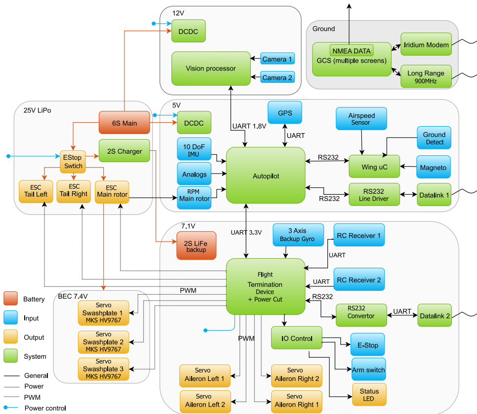
Figure 6.14: Schematic overview of the DelftaCopter electronics
