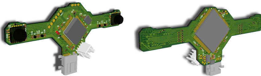
(a) Front side with dual TCM8230MD and STM32F4 (b) Back side with MAX II CPLD
