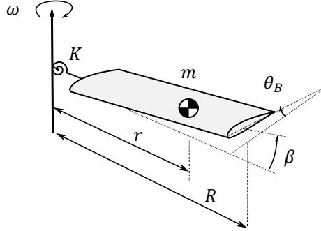
Figure 5.3: A simplified rigid rotor model turning with an angular rate \omega , with mass m , radius R and spring stiffness K and yielding a flapping angle \beta and blade pitch angle or rotor feathering angle \theta_B .
