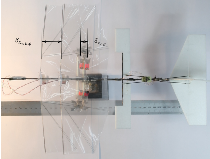
Figure 3.5: Photos of the wing configurations for hover and fast flight superimposed on each other. The DelFly LiMo is balanced on red supports under each wing to show the longitudinal location of the center of gravity. When the wing is shifted forward, the cg also shifts forward with \delta x_{c.g.} . The change in position of the main wing \delta x_{wing} is visible by the difference in location of the wing leading edges.
