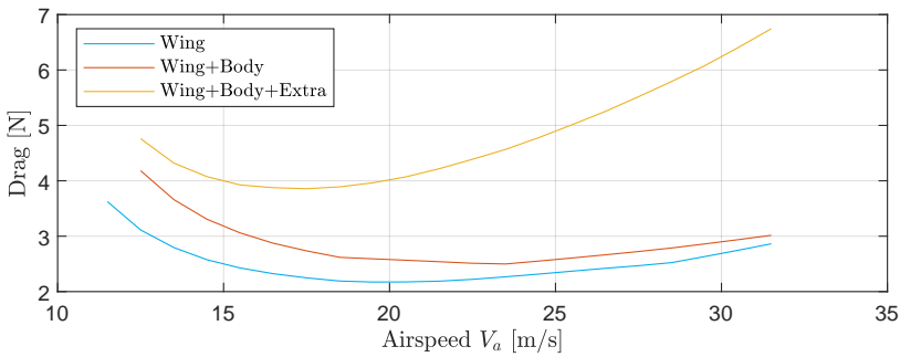
Figure 6.9: The total aerodynamic drag in function of airspeed V_a . When compared to the available thrust from the propulsion from Figure 6.3, one can see that at about 25 m/s the drag becomes larger than 5 N while the maximal achievable thrust with any blade setting becomes lower than 5 N. If the real drag of a built prototype is higher, this will reduce the maximal speed.
