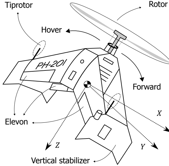
Figure 7.7: The DelftaCopter tail-sitter UAV has a single main rotor that points up and provides lift during hover. Two tip props provide counter-torque in hover, and the swashplate gives lateral and altitude control. In forward flight, the entire vehicle tilts 90° down, and the rotor provides thrust while the biplane delta-wings provide lift, and the elevons provide most of the control.
