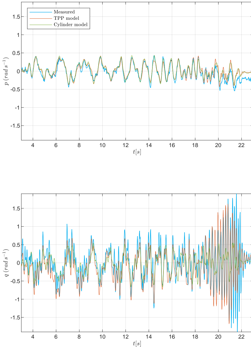
Figure 7.10: Validation chirp on the elevator axis in forward flight. The roll response p (yaw in fixed-wing aircraft reference frame) is fitted accurately by both TPP and CD models, while in the pitch response q , the TPP models start to show significant difference around 20 s and the CD model is unable to replicate those frequencies at all.
