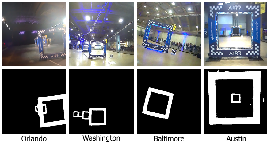
Figure 9.6: Qualitative results of the generated segmentation masks by the final GateNet model from onboard images of each of the events.
