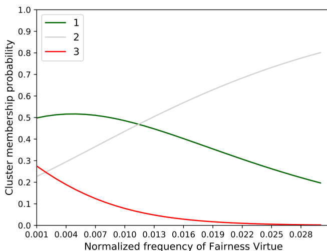
Figure 2.6: Cluster membership prediction: fairness virtue.
