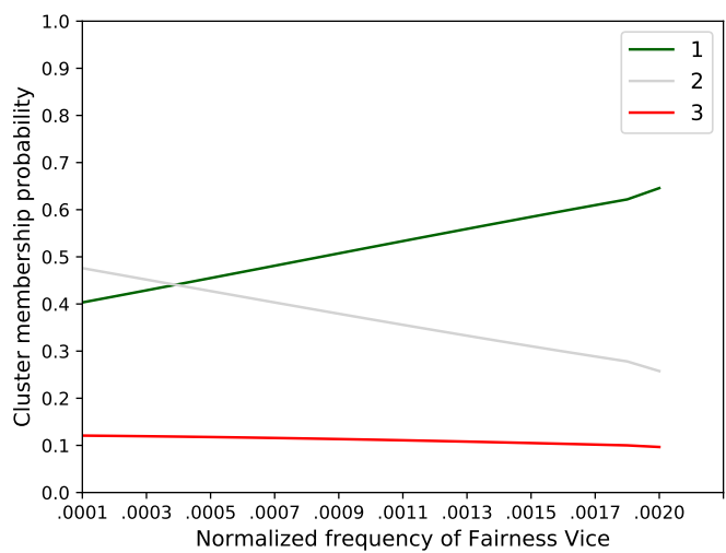
Figure 2.4: Cluster membership prediction: fairness vice.
