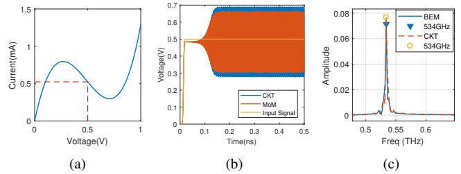
Fig. 2. (a) The I-V characteristic of the RTD with the bias point shown in dashed lines (b) Self-sustained voltage oscillations at the output port (across the tunnel gap). (c) The spectrum of the voltage oscillations
