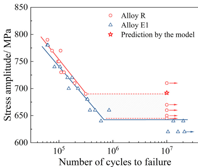
Fig. 5. Rotating bending S-N data for Alloy R and the corresponding closest reference steel Alloy E1. The fatigue data for Alloy E1 were taken from the NIMS database.
