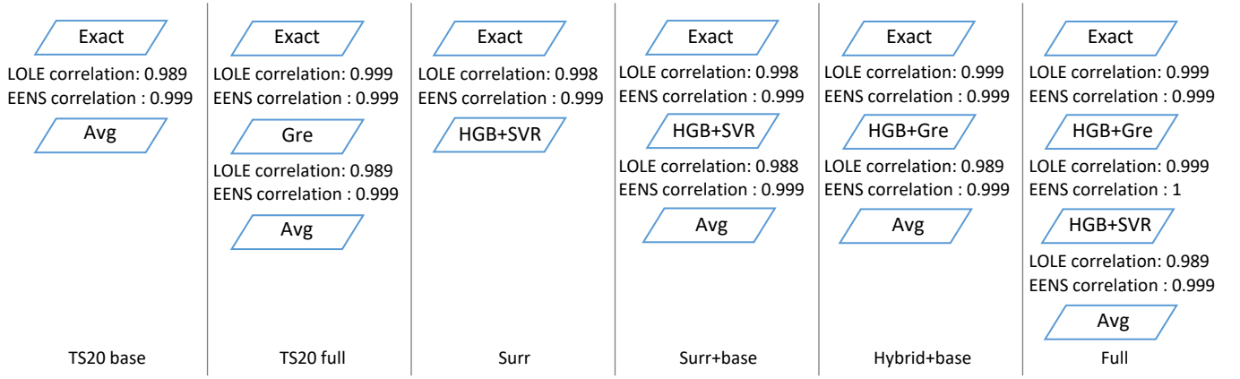
Fig. 1. MLMC model combinations used. Level-to-level sample correlations for LOLE and EENS are indicated.
