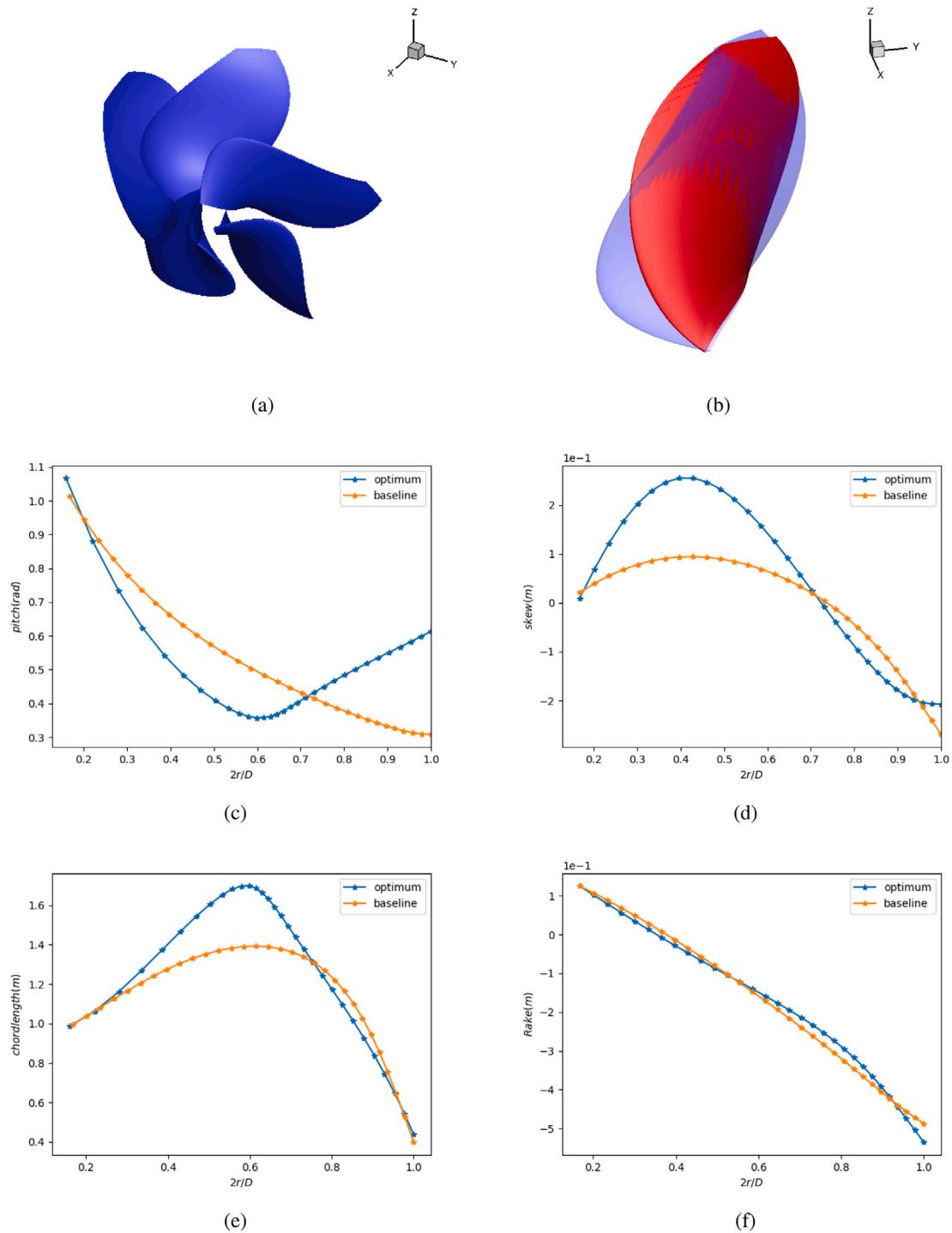
Fig. 17. Design solution with minimum suction side cavitation volume: (a) geometry, (b) comparison with baseline geometry, (c) pitch distribution of baseline and design, (d) skew distribution of baseline and design and, (e) chordlength distribution of baseline and design and, (f) rake distribution of baseline and design.
