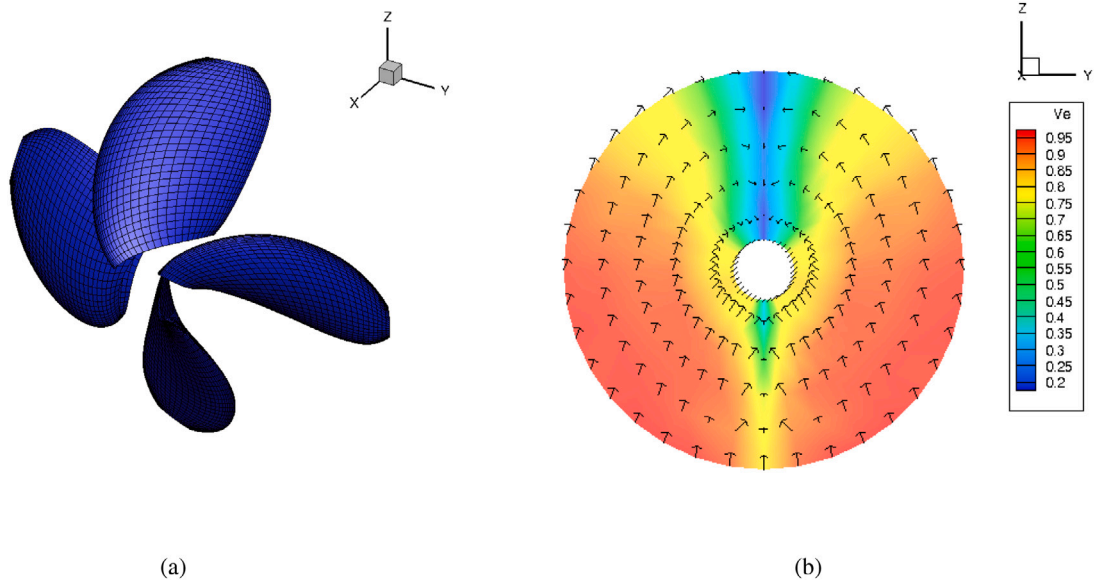
Fig. 2. (a) Wageningen B4-70 propeller base geometry and (b) Effective wakefield of Seiun-Marvessel, V_e = \sqrt{V_x^2 + V_y^2 + V_z^2} . The wakefield was provided by MARIN for this research and is available on request.
