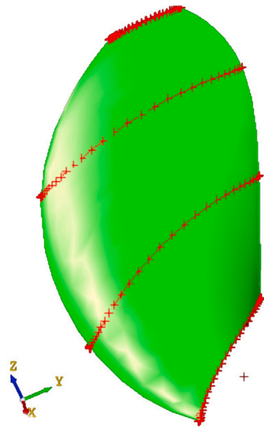
Fig. 3. Blade hydrofoils.
