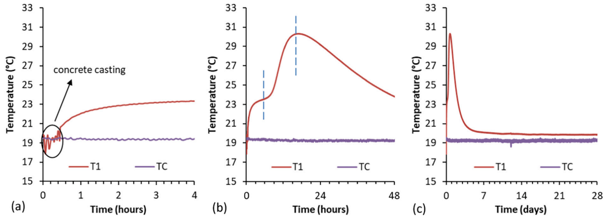
Fig. 7. Temperature evolution of AASC in ADTM1 in 4 h (a), 48 h (b) and 28d (c).
