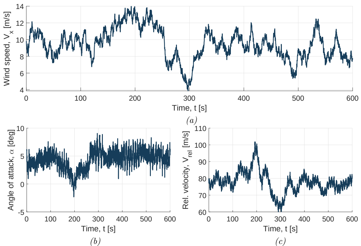
Figure 2. (a) Turbulent inflow of class A with a reference wind speed of 10\text{m/s} . (b) Corresponding angle of attack variation at r/R = 0.97 . (c) Corresponding relative velocity experienced by the blade at r/R = 0.97 .
