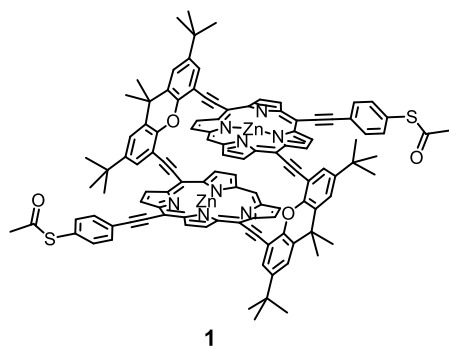
Figure 1. Chemical structure of the target compound 1 .
