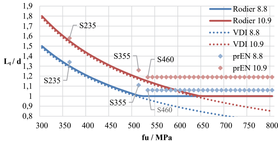
Figure 5 Minimum thread engagement length by Rodier [7], VDI 2230 [20] and prEN [25] for through threaded hole for different bolt hole material grade
