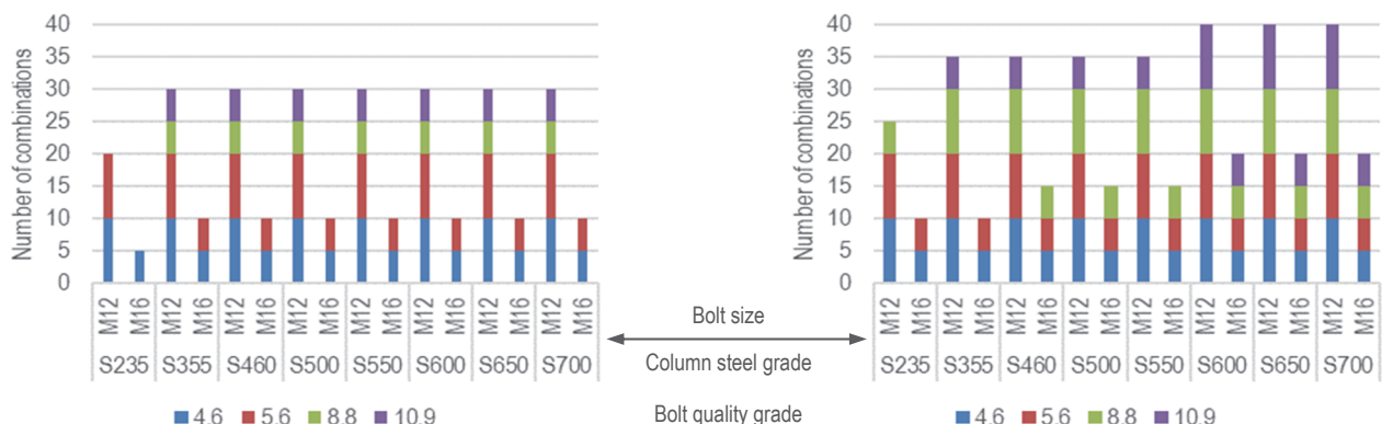
c) prEN [25] influence of bolt size and column steel quality grade for different bolt quality grades
