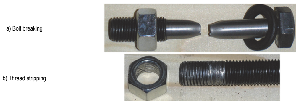
Figure 4 Bolt failure [21]
