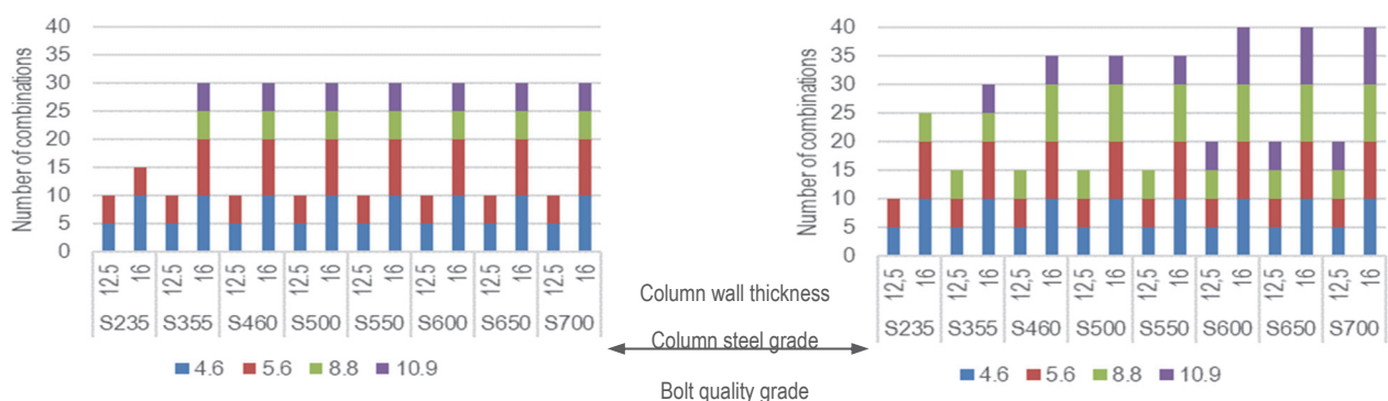
a) prEN [25]-influence of column wall thickness and column steel quality grade for different bolt quality grades
