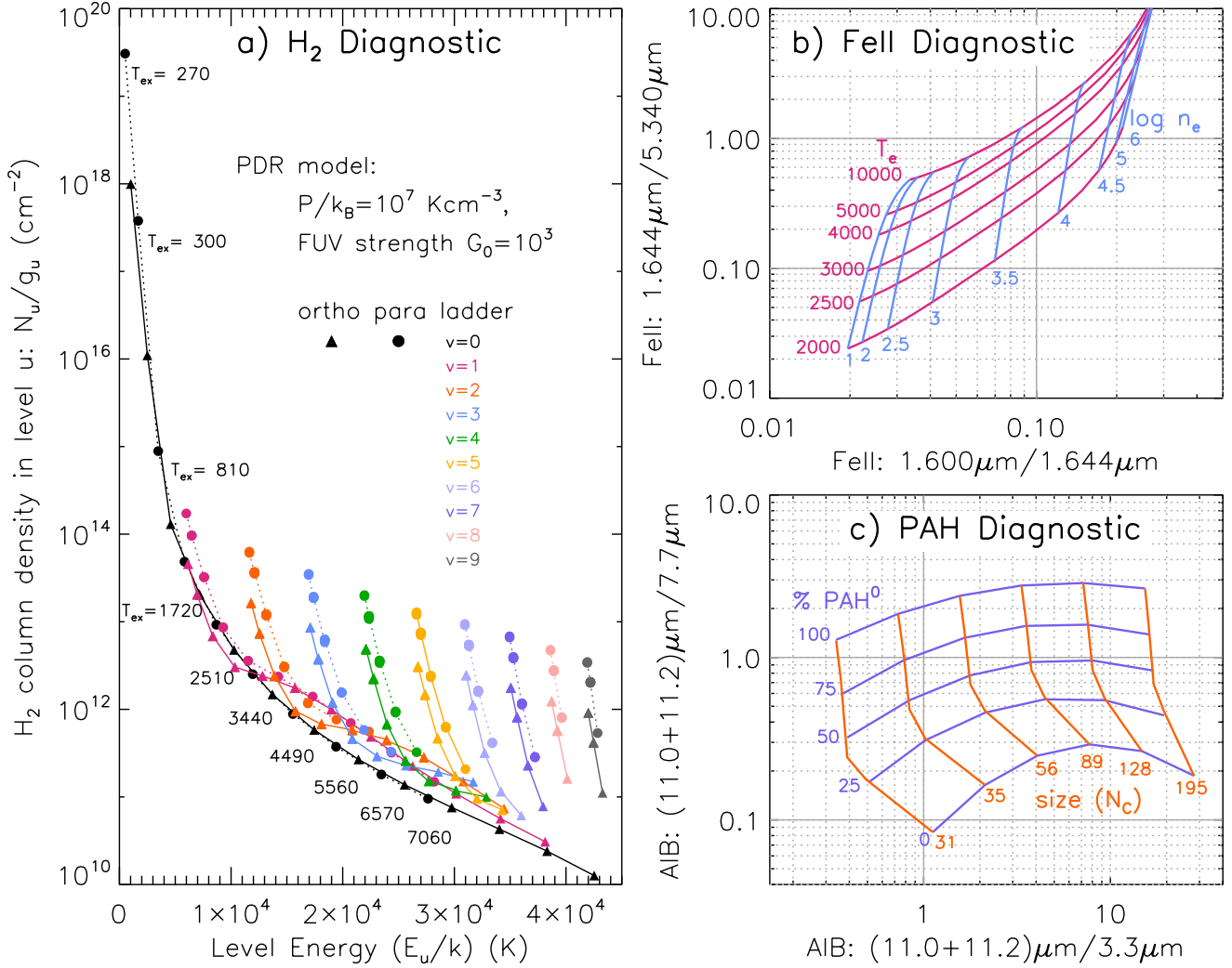
Figure 4. Example IR PDR diagnostics: (a) Excitation diagram from \text{H}_2 lines in PDRs, that are observable by MIRI and NIRSpec, as a tracer of the warm and hot (UV-pumped) excitation temperatures (excitation temperatures derived from the level populations by a local Boltzmann fit are indicated); (b) The [\text{Fe II}] lines as a tracer of the temperature and density distribution from the ionized gas to the PDR (Del Zanna et al. 2021 and using atomic data from Deb & Hibbert 2011 and Smyth et al. 2019); (c) AIB emission ratios as a tracer of PAH size (in function of the number of carbon atoms, N_c ) and charge (in function of the neutral PAHs fraction, i.e., \text{PAH}^0/(\text{PAH}^0 + \text{PAH}^1) ), computed from harmonic IR spectra using PAHdb and assuming an interstellar radiation field (see Section 8 for a description of PAHdb). Figure adapted from Maragkoudakis et al. (2020).
