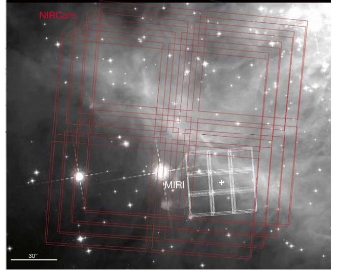
Figure 7. Overlay of the JWST NIRCcam (red) and MIRI (white) imaging footprints on the Hubble Space Telescope image of the Orion Bar at 1.3\ \mu\text{m} (Robberto et al. 2020). MIRI observations are centered on position \alpha = 05\ 35\ 20.3448 and \delta = -05\ 25\ 4.01 (position indicated by the white cross). For NIRCcam, only module B covering the Bar is shown in this overlay. Module A is situated to the North (outside of the image), and the pointing position (also outside this image) is situated in between these two modules at \alpha = 05\ 35\ 20.1963 , \delta = -05\ 23\ 10.45 .
