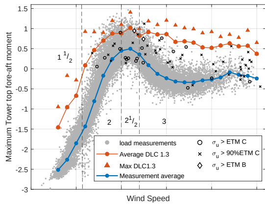
(a) Maximum Tower top fore-aft moment
