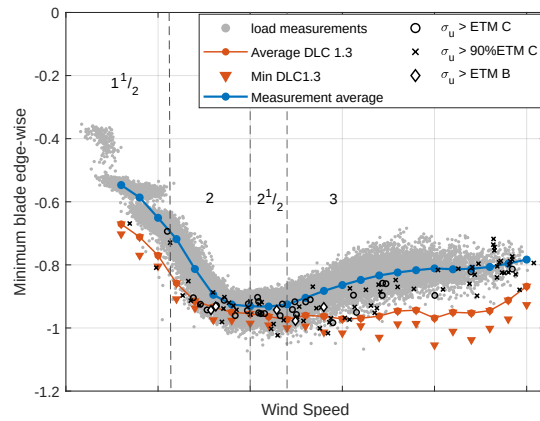
(b) Minimum Blade root edge-wise moment
