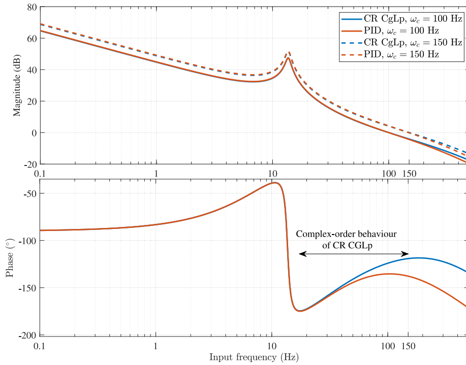
Fig. 19. Bode diagram for a PID and DF diagram of a CR CgLP, showing the complex-order behaviour of CR CgLP. PM for CR CgLP at 100 Hz is 55° and for 150 Hz is 60°. PM for the PID at 100 Hz is 45° and for 150 Hz is 43°.
