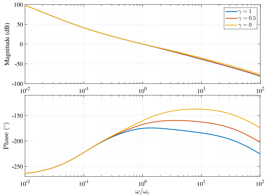
Fig. 8. DF of the open loop system for different \gamma values versus the ration of \omega/\omega_c .
