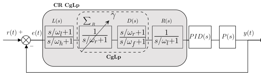
Fig. 7. The control loop used for precision motion control using CR CgLp. P(s) is the plant. PID(s) = k_p (1 + \omega_l/s) \left( \frac{s/\omega_d+1}{s/\omega_z+1} \right) .
