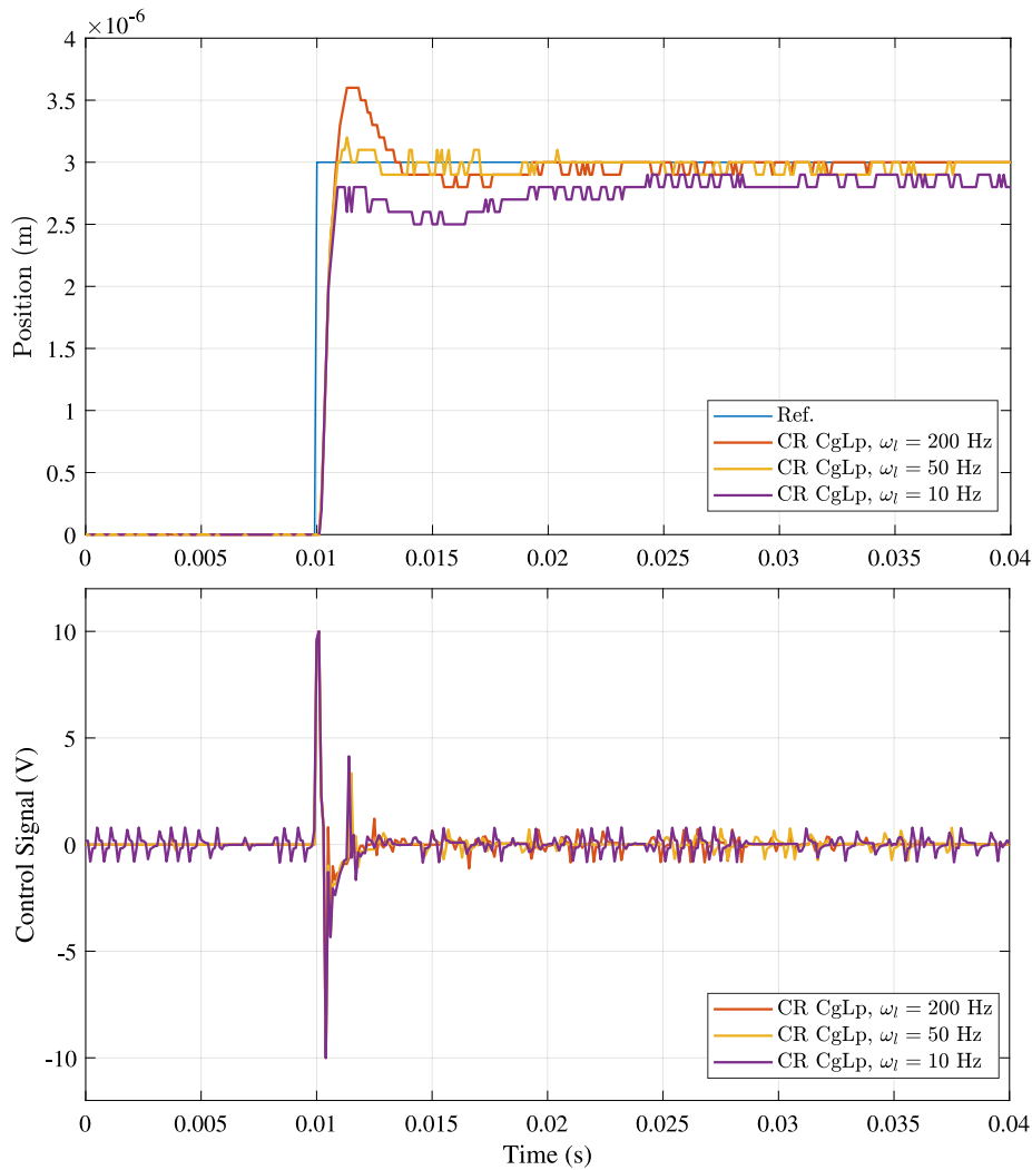
Fig. 18. The effect of varying \omega_l on transient response and its corresponding control signal of the CR CgLp.
