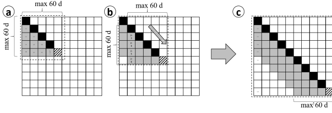
Fig. 2. Computational approach for n SAR acquisitions, where n is increasing in time. (a) Lower triangular matrix showing all possible interferometric combinations in gray, the NWP model realizations in black, and the new atmospheric delay estimate hatched. (b) For growing time series, a maximum temporal baseline of 60 days is used, leading to (c) bandwidth of interferometric combinations.
