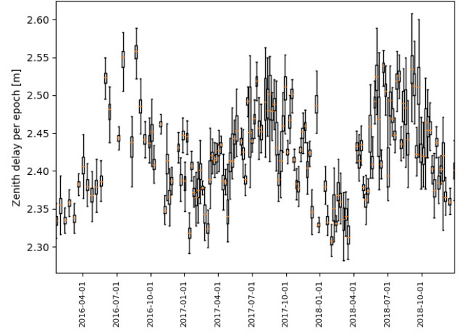
Fig. 8. Estimated topography-adjusted single-epoch zenith delay values \delta_{zenith,h,p}^{ti} as a function of time. The delays are given as box plots for every individual epoch. This shows a seasonal trend in delays, which is due to temperature and moisture changes, as the variation in total air pressure can only explain a minor change in total delay.
