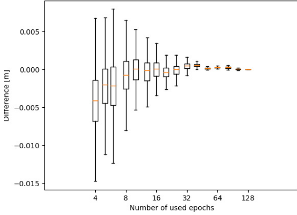
Fig. 13. Difference in result for final atmospheric delay estimation for a different number of acquisitions (epochs), relative to the reference case with 128 images. The box plots express the expected error in the estimated atmospheric delay \hat{\delta}^i due to the use of less acquisitions. Solutions show an average error of less than 1 mm for 40 epochs when we use a 500-m InSAR grid and temporal baseline of 60 days.
