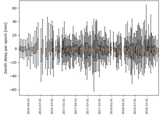
Fig. 9. Spread of difference between NWP model delays \delta_{NWP,zenith,p}^{ti} and estimated single-epoch delays \delta_{zenith,p}^{ti} per acquisition. The delay differences are given as box plots for every individual epoch. This shows that the differences in the summer tends to be larger than in winter.
