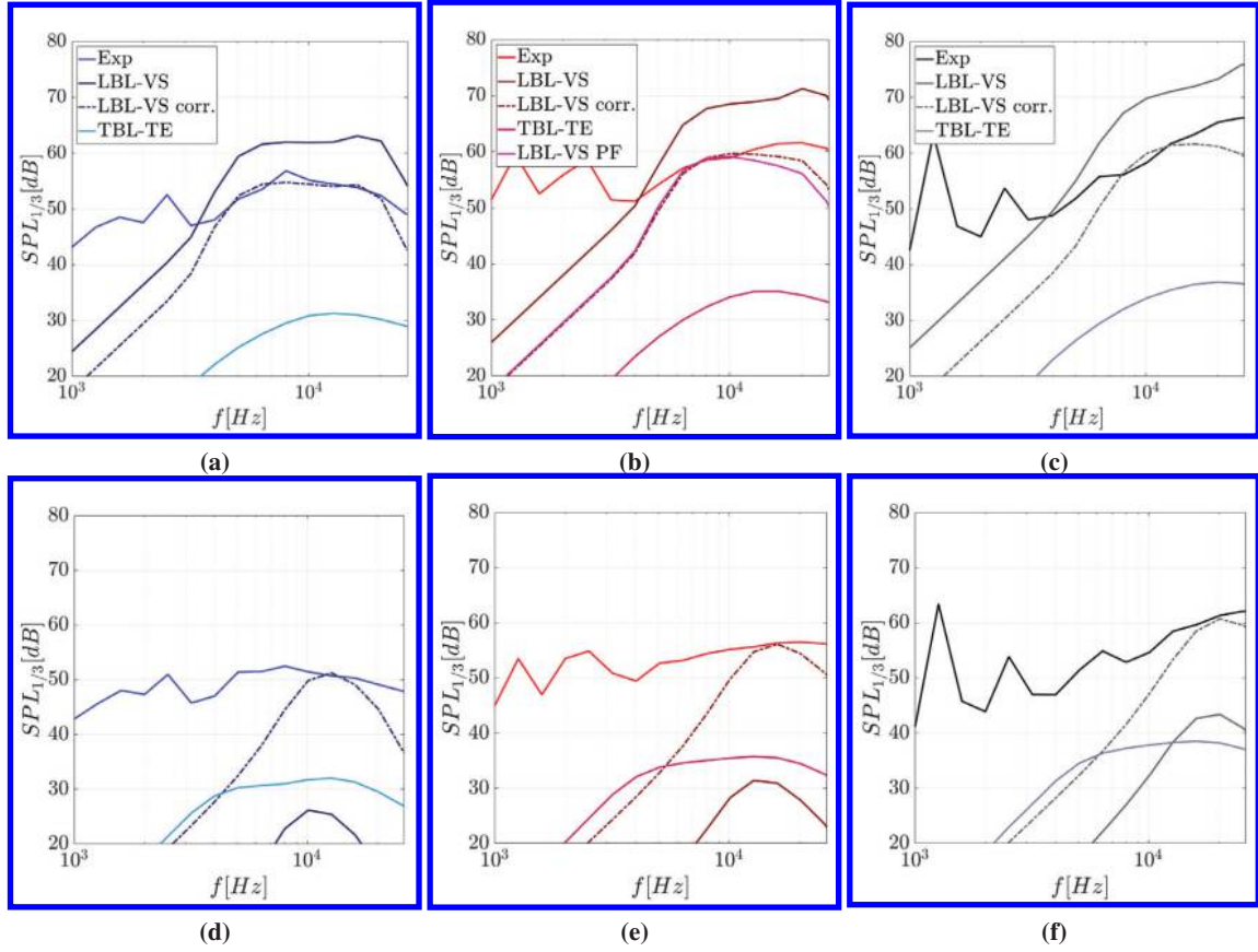
Fig. 14 Comparison at mic 2 between the experimental noise spectra and the numerical predictions at J = 0.6 and 4000 rpm (a), J = 0.6 and 5000 rpm (b), J = 0.6 and 6000 rpm (c), J = 0.4 and 4000 rpm (d), J = 0.4 and 5000 rpm (e), J = 0.4 and 6000 rpm (f).
