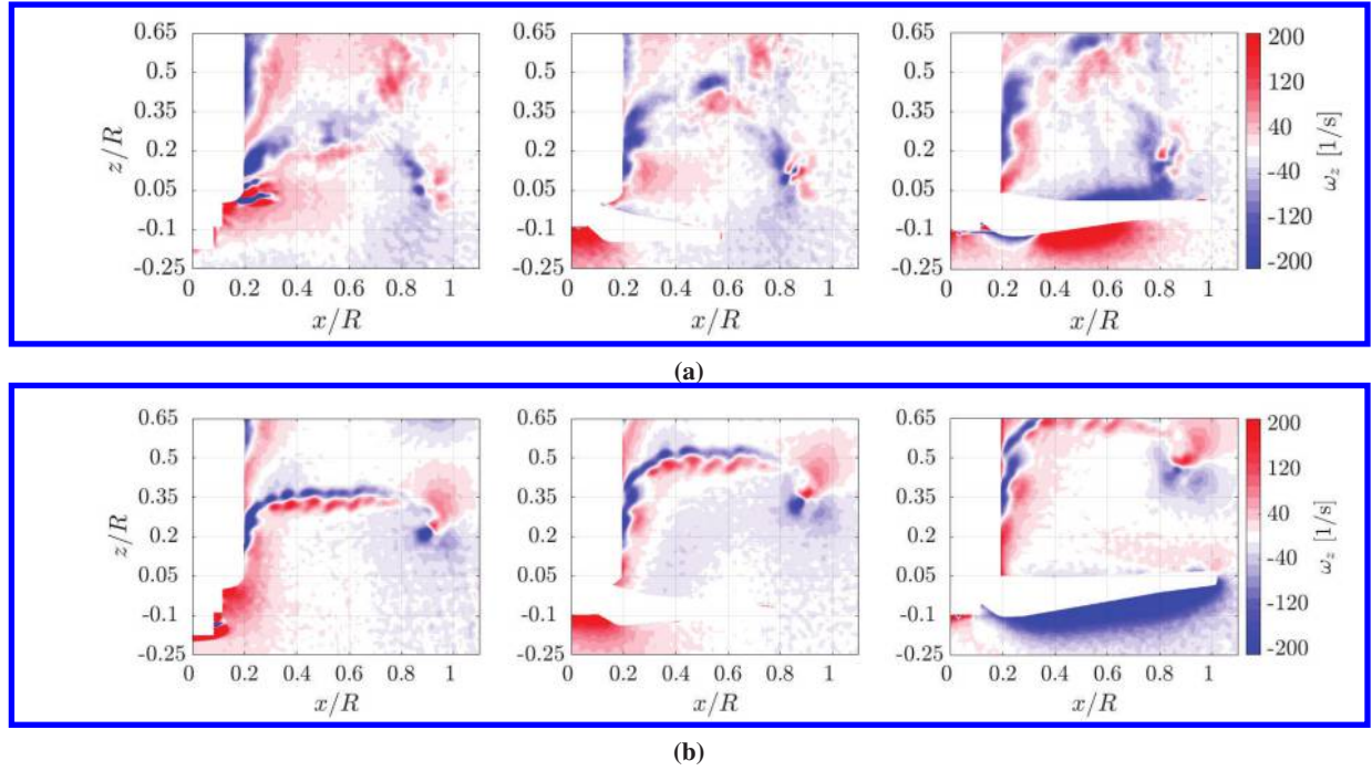
Fig. 8 Instantaneous vorticity distribution in the wake at 4000 rpm and J = 0 (a) and J = 0.4 (b). The three columns represent three different propeller phases: \phi = 0^\circ , \phi = 45^\circ , \phi = 90^\circ (from left to right)
