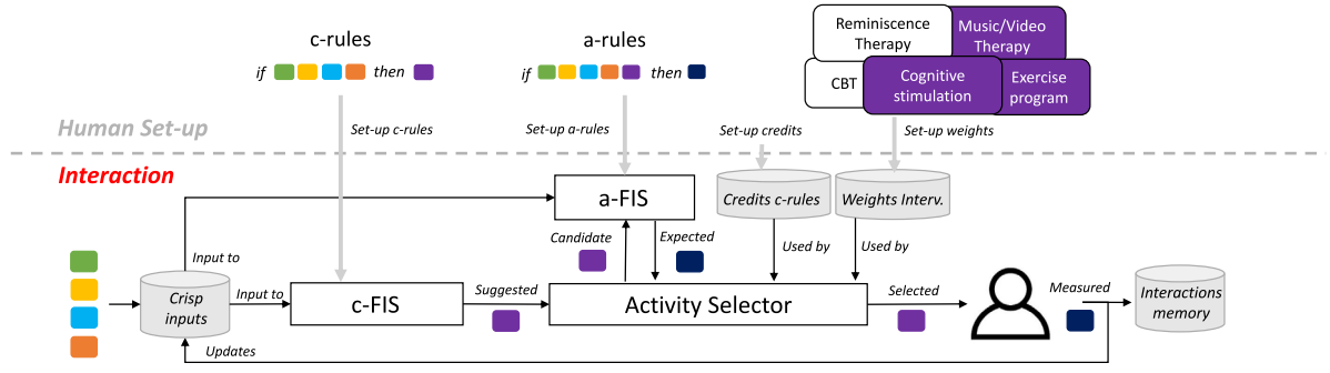
Fig. 1. Overview of the proposed framework. The colored input boxes indicate four of factors relevant in dementia care and that can be used as input for the FISs. Purple boxes indicate possible activities of the robot, and dark blue ones indicate feedback measures.
