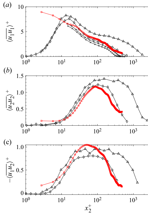
Figure 5. Semi-logarithmic plots of the wall-normal profiles of the normalized Reynolds stress components: (a) \langle u_1 u_1 \rangle^+ , (b) \langle u_2 u_2 \rangle^+ , and (c) -\langle u_1 u_2 \rangle^+ . Present data: red squares denote Re_\theta = 850 . Literature results: from De Graaff & Eaton (2000), diamonds denote Re_\theta = 1430 , and triangles denote Re_\theta = 5200 ; from Erm & Joubert (1991), \times symbols denote Re_\theta = 697 , and + symbols denote Re_\theta = 1003 .
