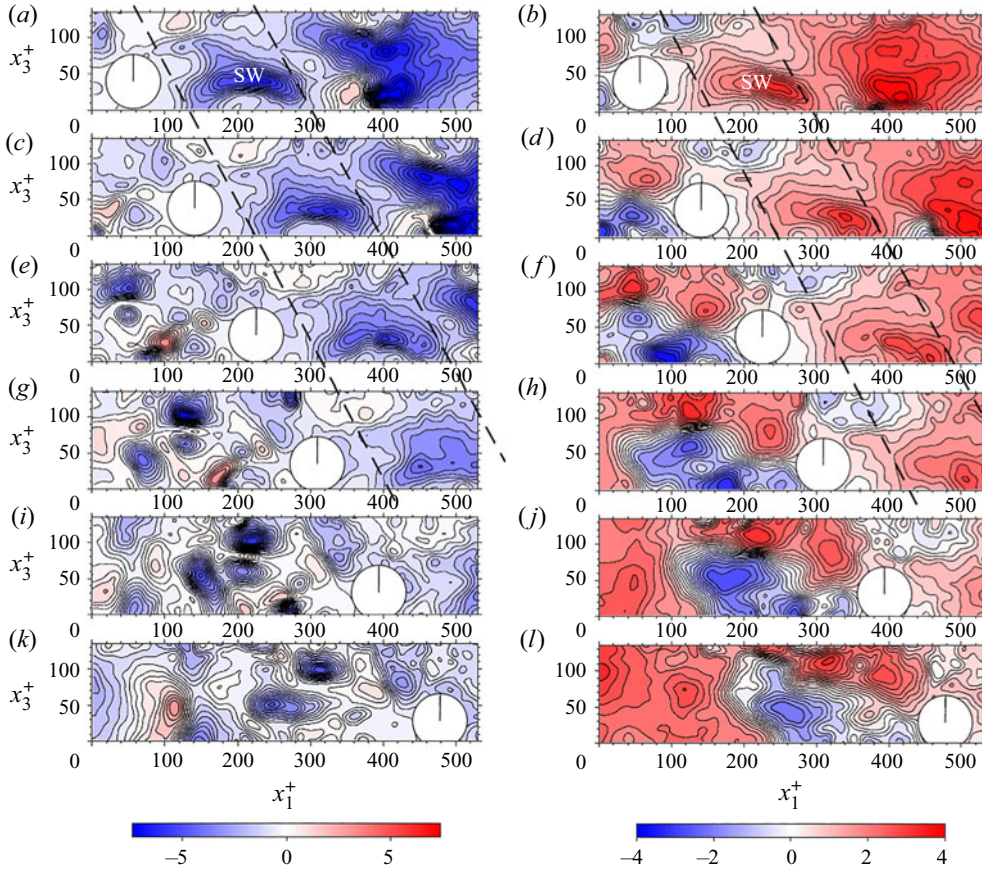
Figure 21. For S_4 , a sequence ( \Delta t^+ = 4.9 ) of equatorial wall-parallel planes depicting the correlations of the instantaneous water fluctuating velocities (u_1 u_2)^+ ( a, c, e, g, i, k ), and the streamwise water fluctuating velocities u_1^+ ( b, d, f, h, j, l ). The hydrogel sphere is superposed as a filled white circle. Its initial orientation is indicated by a dashed line, while its changing orientation is indicated by a solid line. A progressing sweep motion (SW) can be seen between the two parallel dashed lines in ( a-h ). Note that the view is from the wall upwards.
