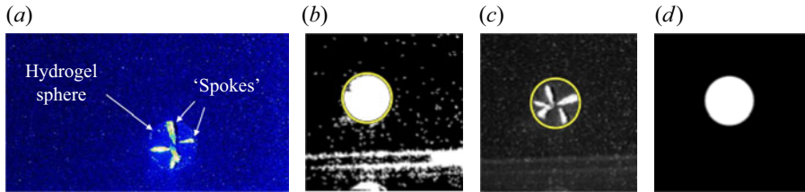
Figure 2. Overview of the sphere detection procedure. Cropped images (single camera) of: (a) raw PIV data showing the spokes imaged within the hydrogel sphere and the tracer particles in its vicinity; (b) silhouette enhanced (and ‘holes’ filled) sphere. The sphere’s perimeter was detected using the circular Hough transform and is indicated by a yellow circle in (b,c). (c) Detected sphere perimeter containing the ‘spokes’. (d) Generated binary mask.
