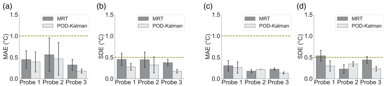
FIGURE 6 MAE and SDE of filtered MR thermometry and Kalman filtered temperature prediction in each probe location and phantom. (a) and (b) present the MAE and SDE from phantom 1, and (c) and (b) show the MAE and SDE from phantom 2. The error lines show the standard deviation from all experiments, and the height of the bars represents the average within the experiments. The dashed green line represents the acceptable MAE and SDE. The bar graphs in (a) and (b) are concerning to six experiments, while the bar graphs in (c) and (d) are regarding to two experiments
