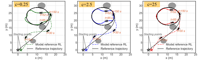
Fig. 13. Collision avoidance performance at different c 's.
